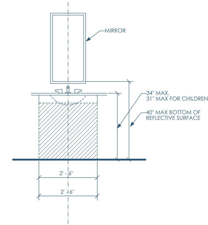
2C/A750 ADA - LAVATORY - FRONT 1/2"=1'-0"
