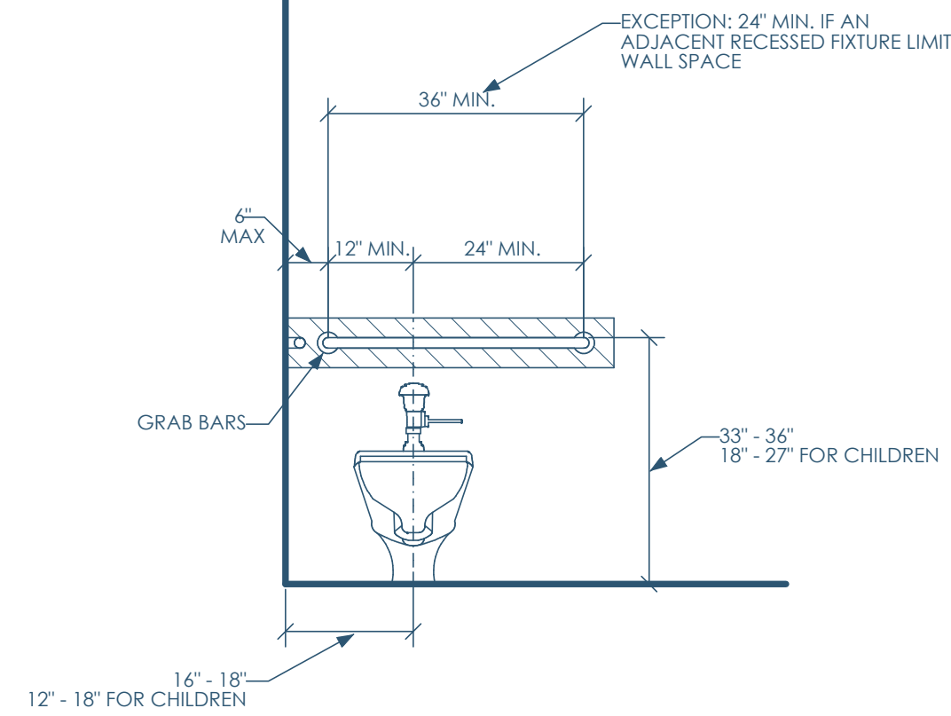
4B/A750 ADA - WATER CLOSET - FRONT 1/2"=1'-0"
