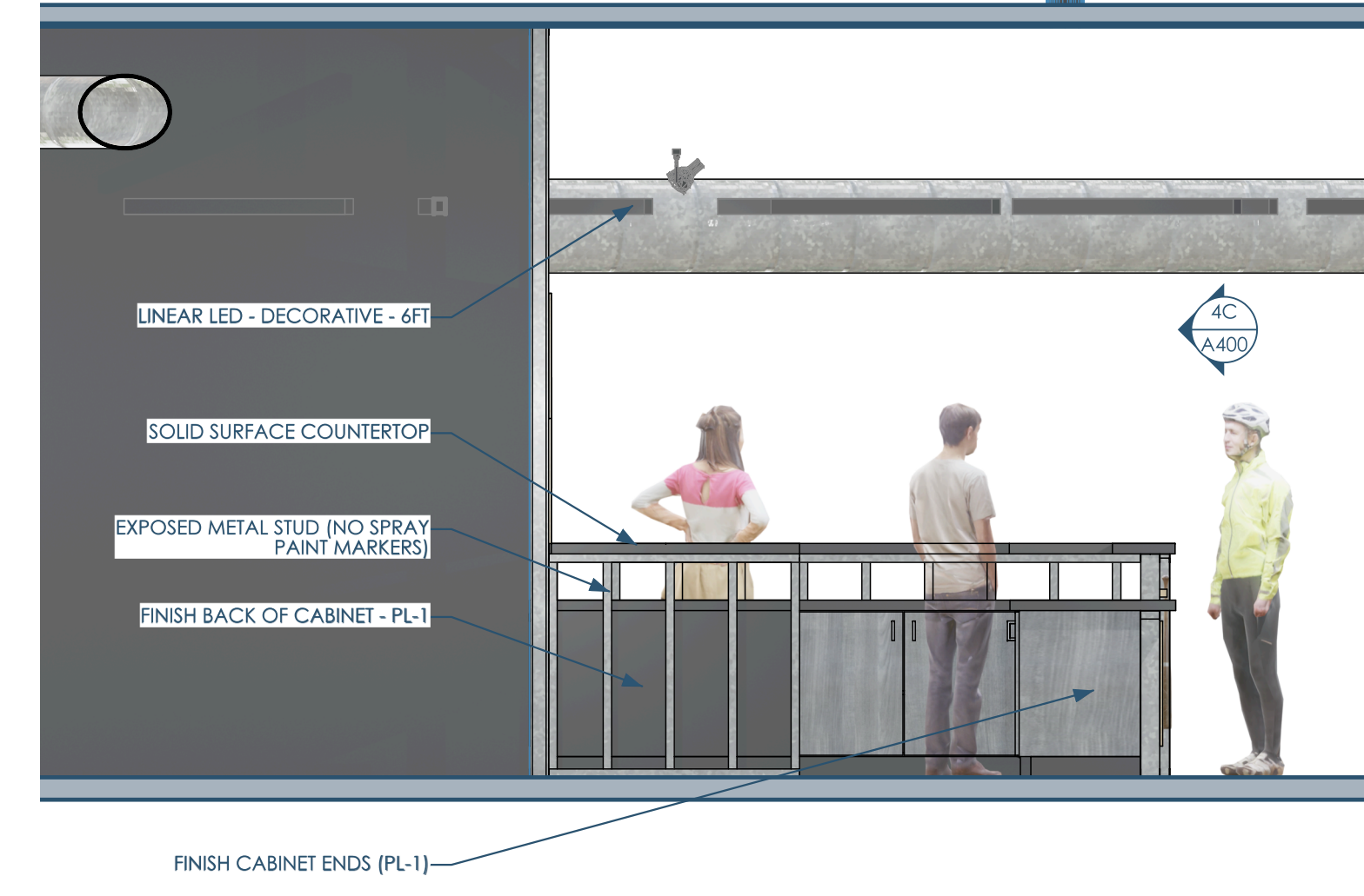
2C/A400 POS - ELEVATION - EAST 3/8"=1'-0"
