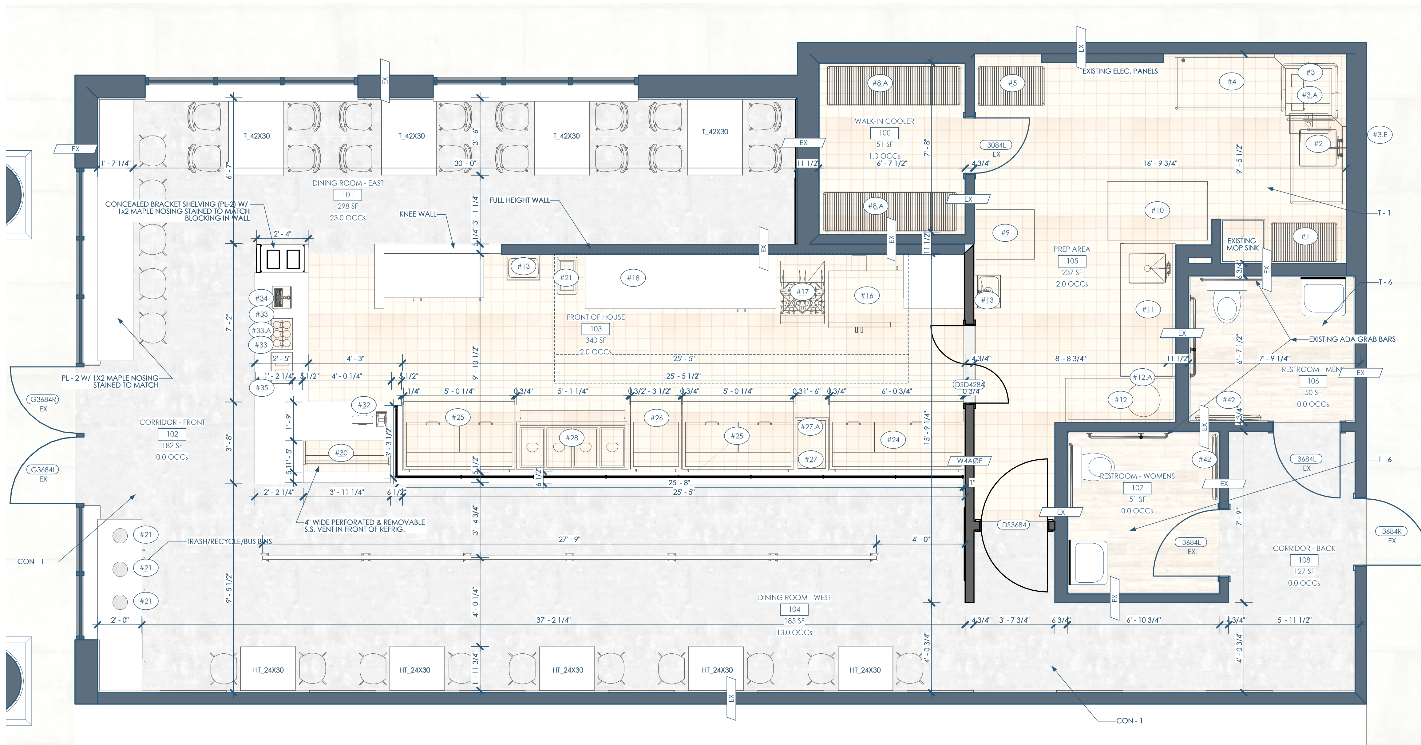
5B/EQ-L EQUIPMENT PLAN - LAYOUT 3/8"=1'-0"
