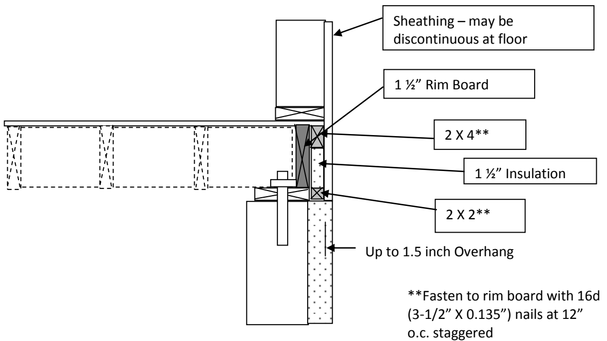
Option 5 – Double Rim Joist With 2X Framing Perpendicular or Parallel to Foundation Wall
