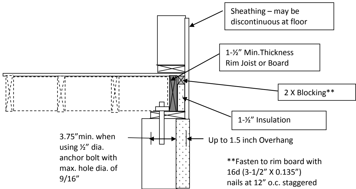
Option 4 – Double Rim Joist With 2X Framing Perpendicular or Parallel to Foundation Wall
