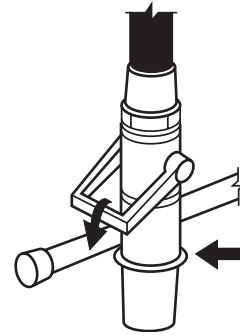
FIGURE A.7.6.2(e) Nozzle in Holder.
