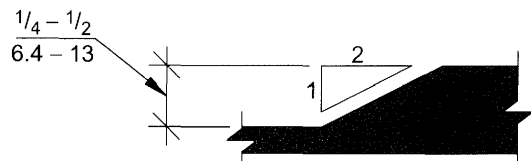
FIG. 303.3 BEVELED CHANGES IN LEVEL
