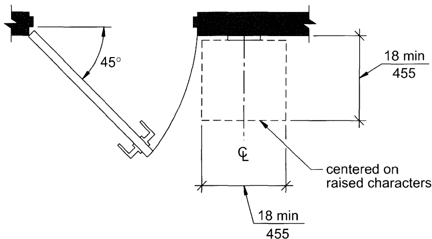
FIG. 703.3.11 LOCATION OF SIGNS AT DOORS
