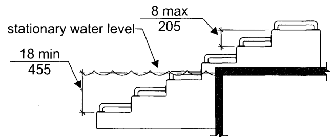
FIG. 1109.5.4 TRANSFER STEPS
