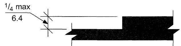
FIG. 303.2 CARPET ON FLOOR SURFACES
