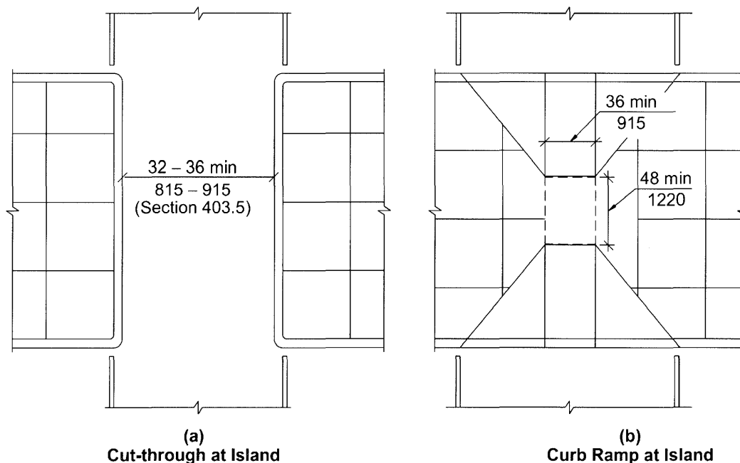
FIG. 406.11 ISLANDS
