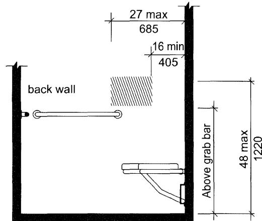
With Seat FIG. 608.4.2 STANDARD ROLL-IN-TYPE SHOWER CONTROL AND HANDSHOWER LOCATION
