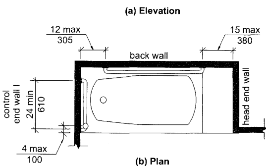
FIG. 607.4.1 GRAB BARS FOR BATHTUBS WITH PERMANENT SEATS
