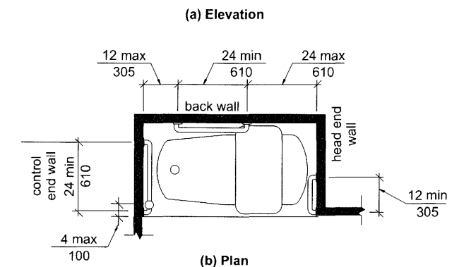
FIG. 607.4.2 GRAB BARS FOR BATHTUBS WITHOUT PERMANENT SEATS
