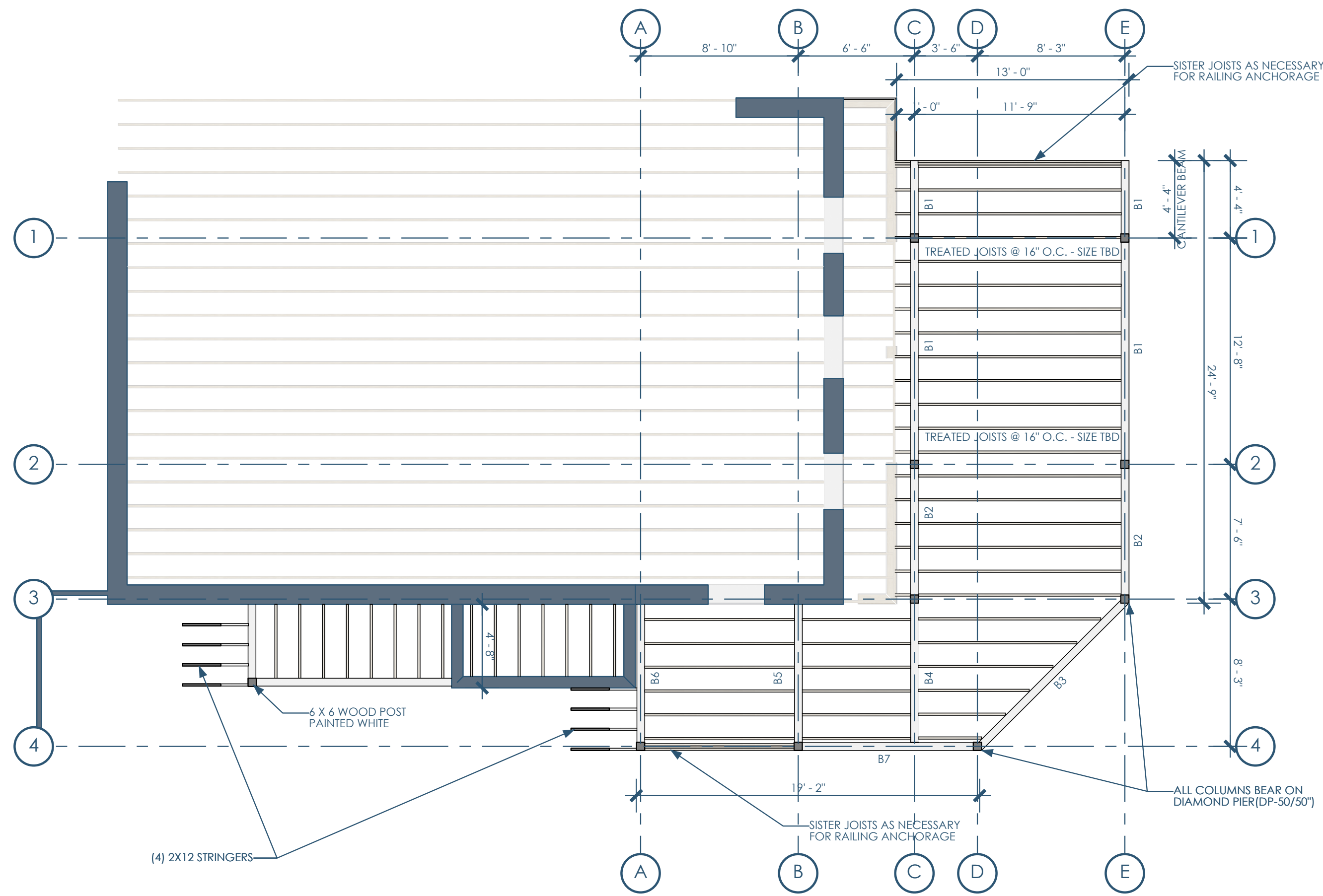
5B/A300 FRAMING PLAN - 1ST FLOOR RCP 3/16\"=1'-0"
