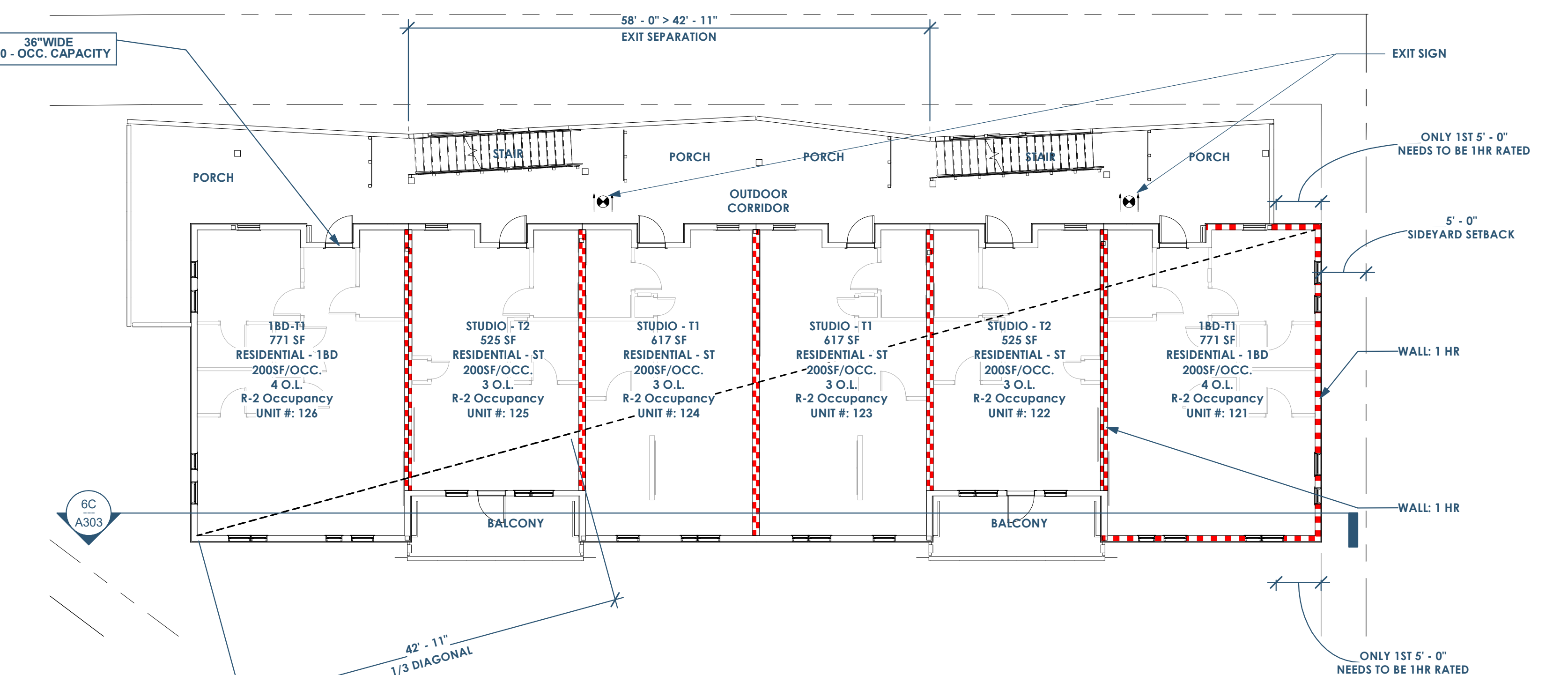
6A LIFE SAFETY - 2ND FLOOR 1" = 10'-0"
