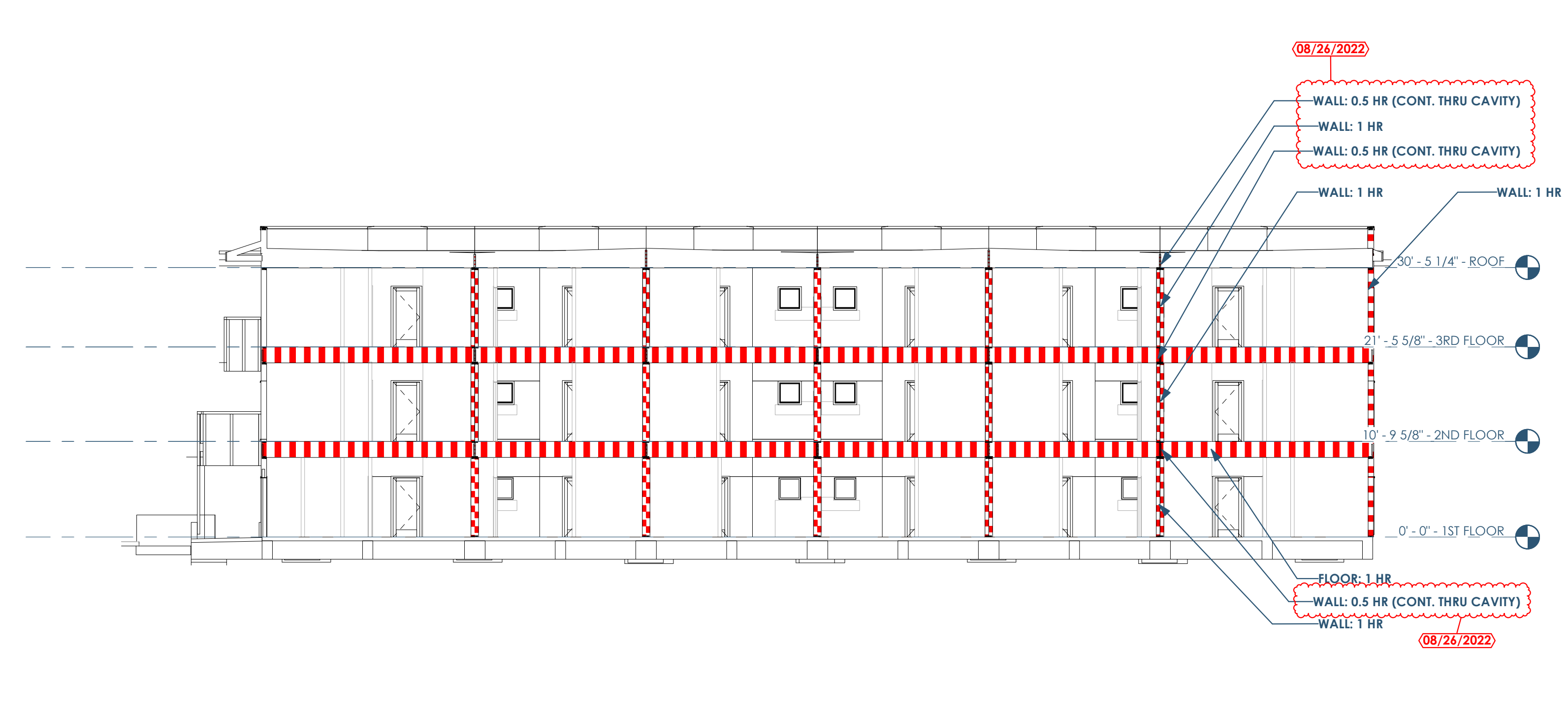
3B LIFE SAFETY SECTION - EAST/WEST 3/32" = 1'-0"
