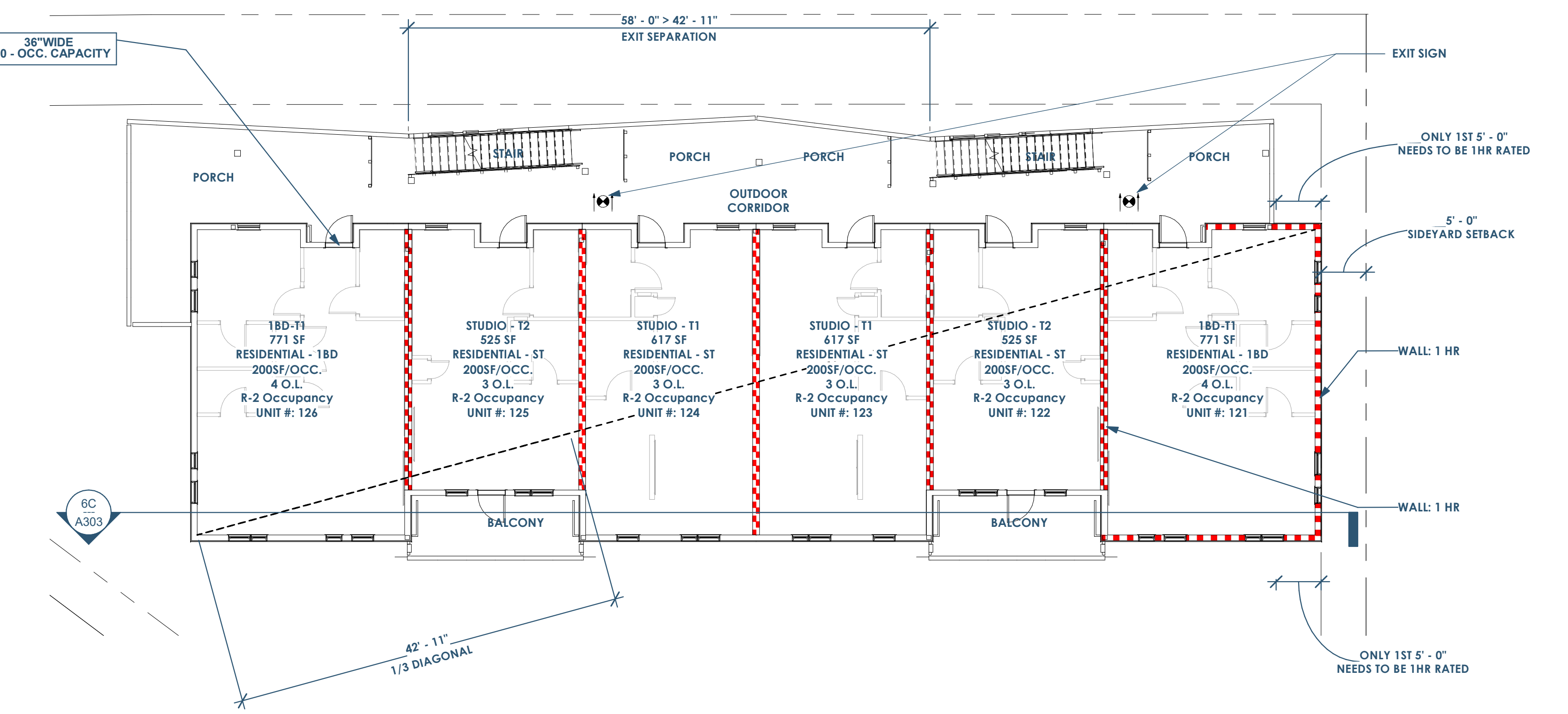
6A LIFE SAFETY - 2ND FLOOR 1" = 10'-0"
