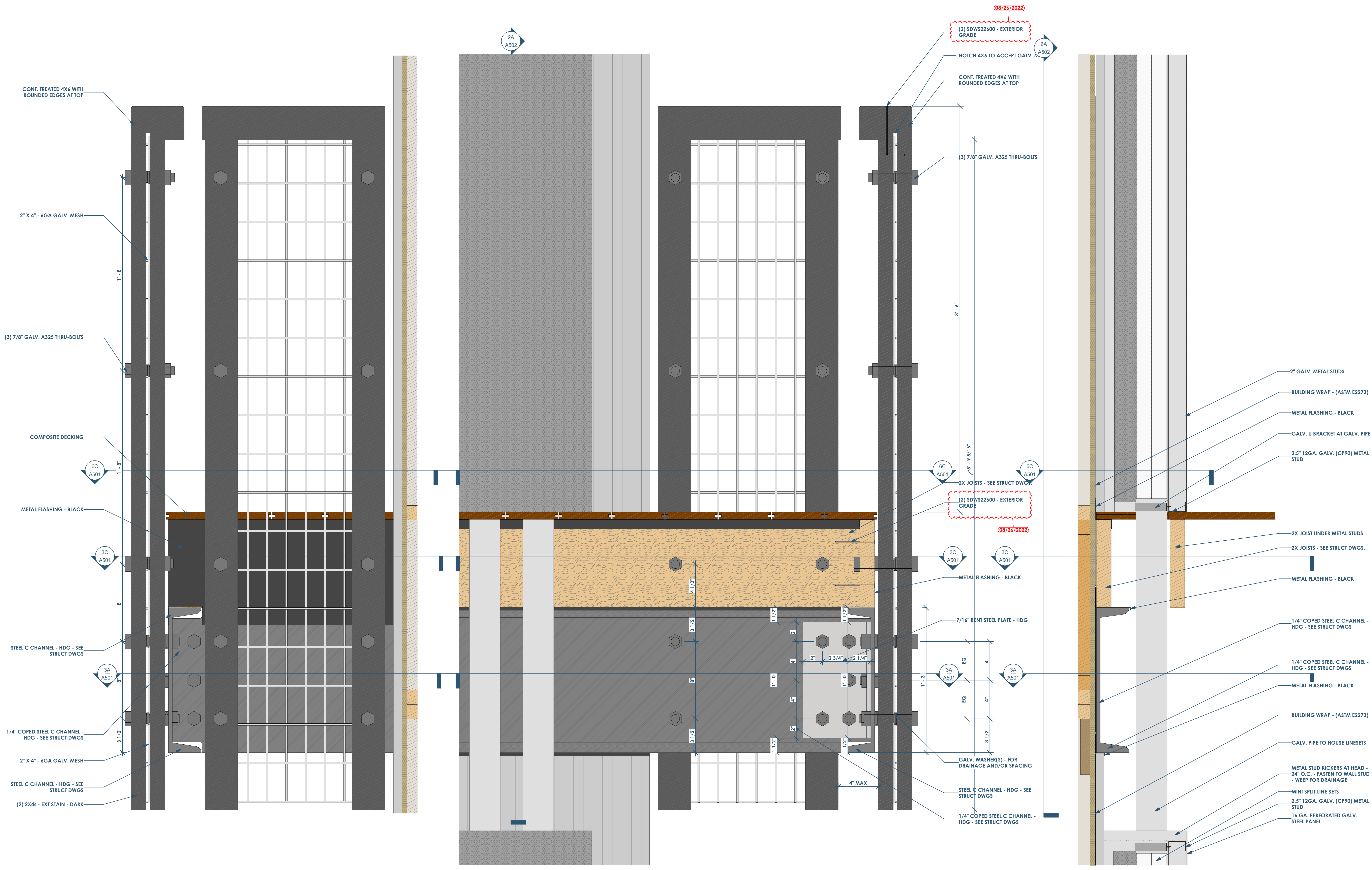
6A A502 SECTION (ELEVATION) DETAIL AT SOUTH BALCONY - LOOKING EAST OR WEST 3" = 1'-0"
