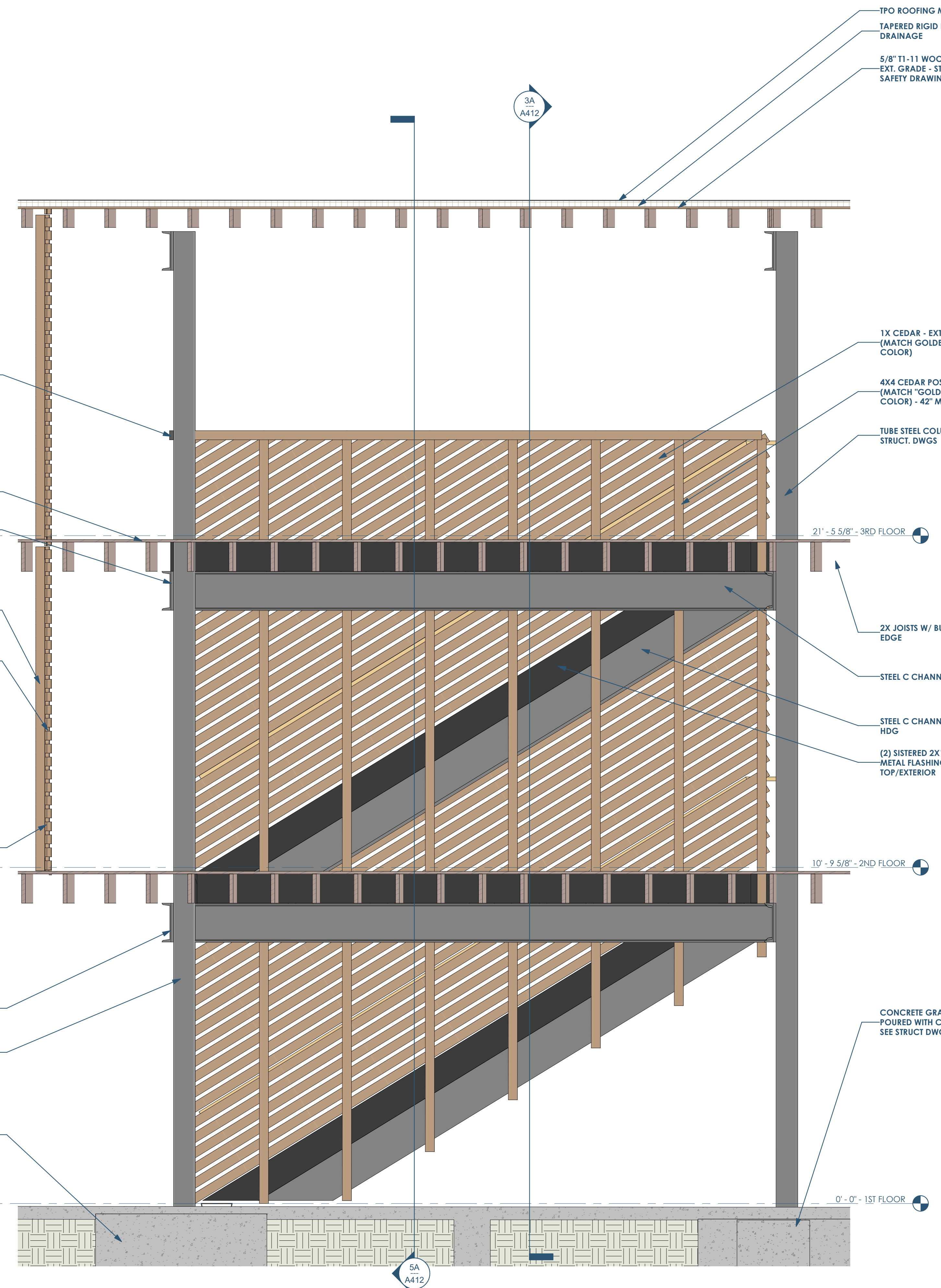
6A A412 STAIR SECTION - CUT THROUGH BALCONY 1/2" = 1'-0"
