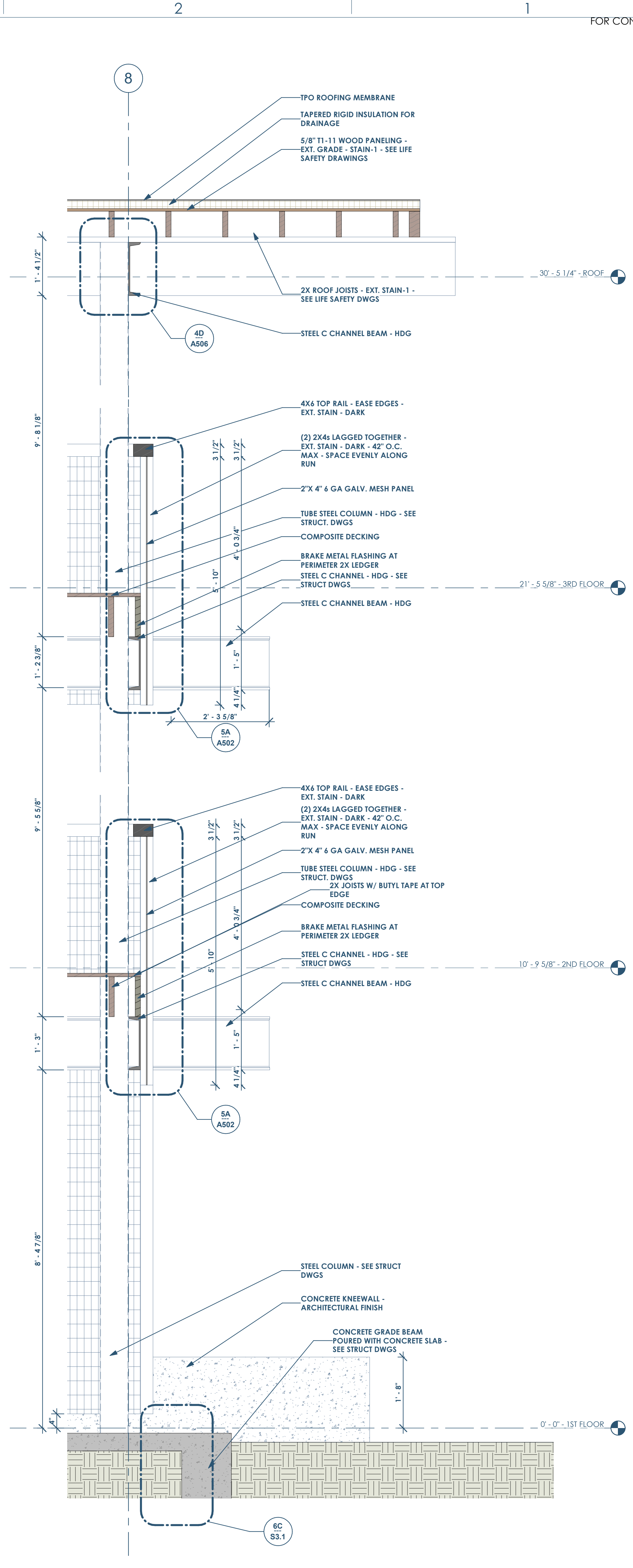
2A WALL SECTION - THRU BALCONY - RAILING 3/4" = 1'-0"
