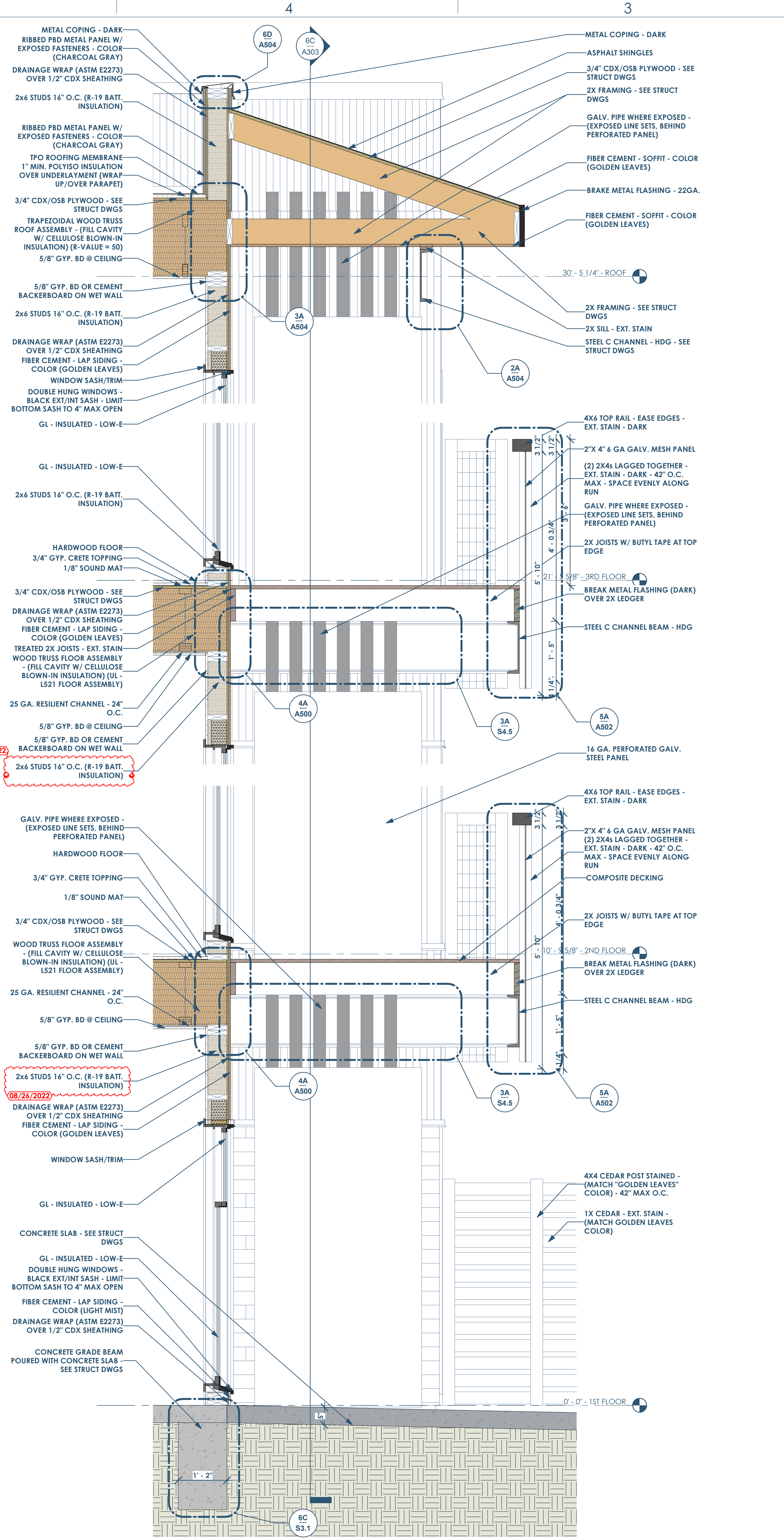
4A WALL SECTION - SOUTH BALCONY 3/4" = 1'-0"
