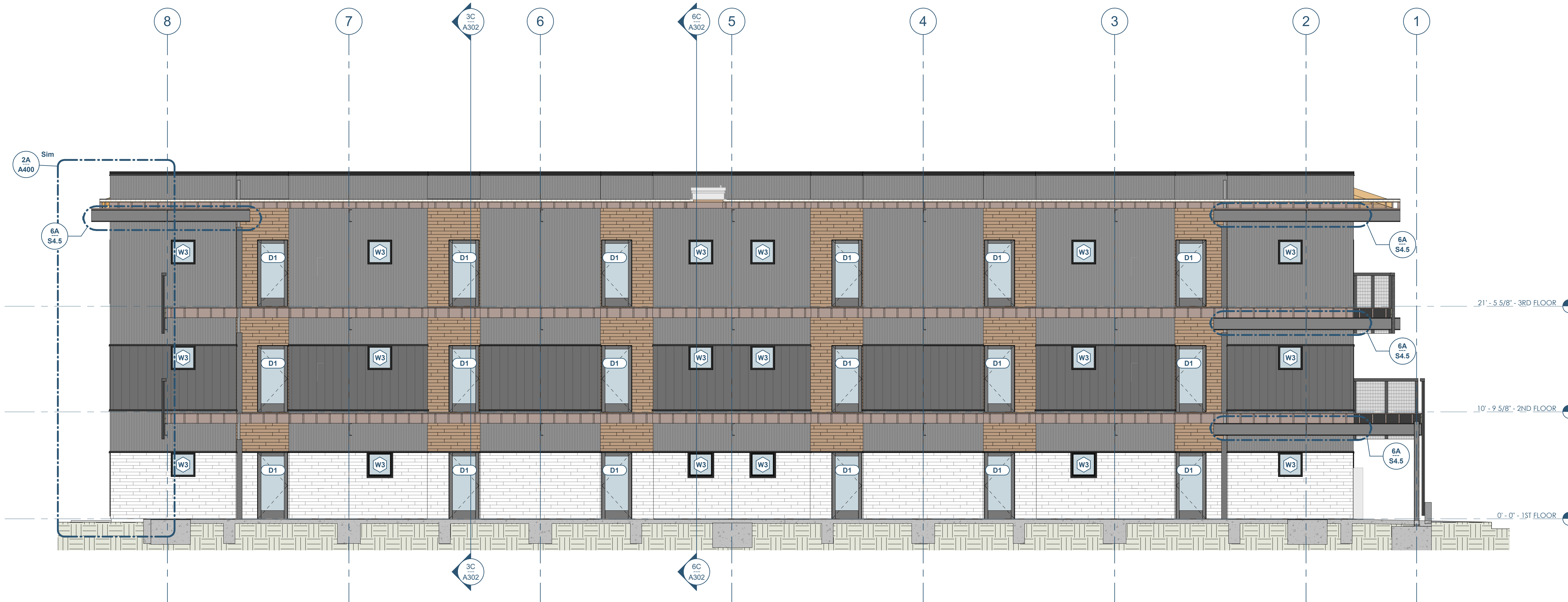
4C A301 BUILDING SECTION - THRU BALCONY - LOOKING SOUTH 3/16" = 1'-0"
