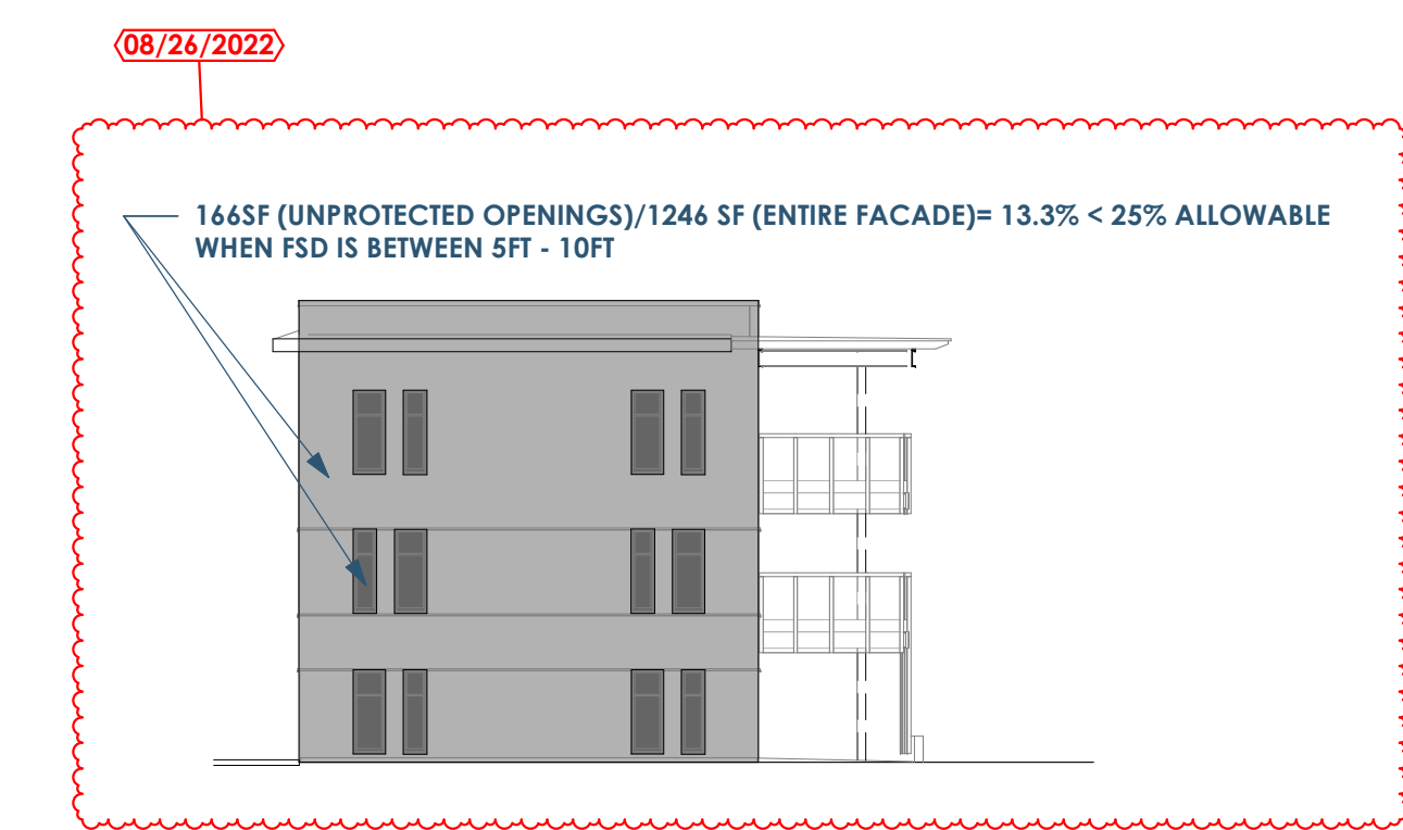
2B A201 DIAGRAMMATIC ELEVATION - EAST 1/16" = 1'-0"
