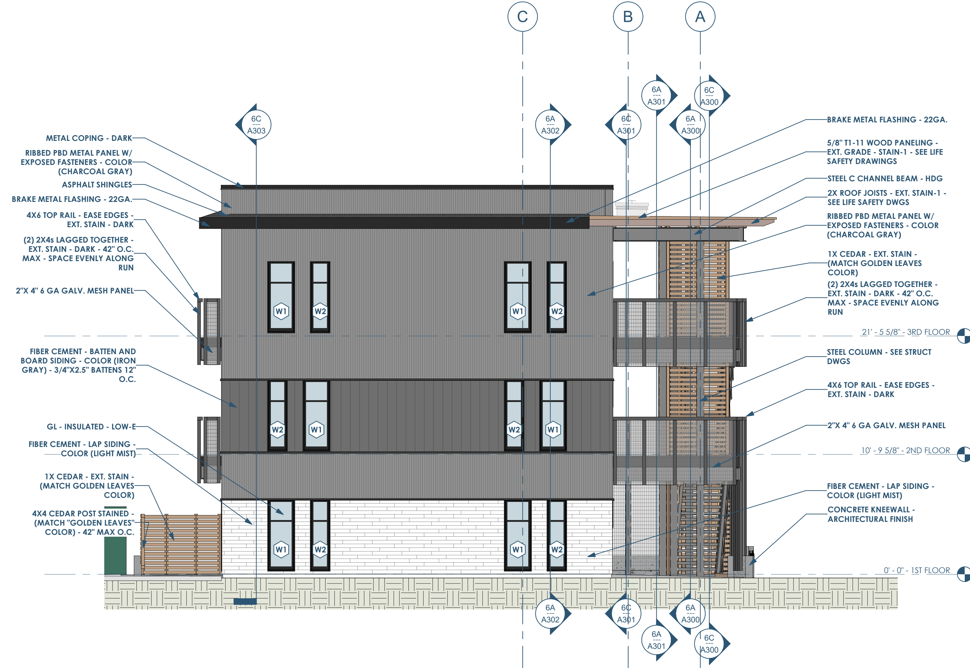
5A A201 BUILDING ELEVATION - EAST 3/16" = 1'-0"
