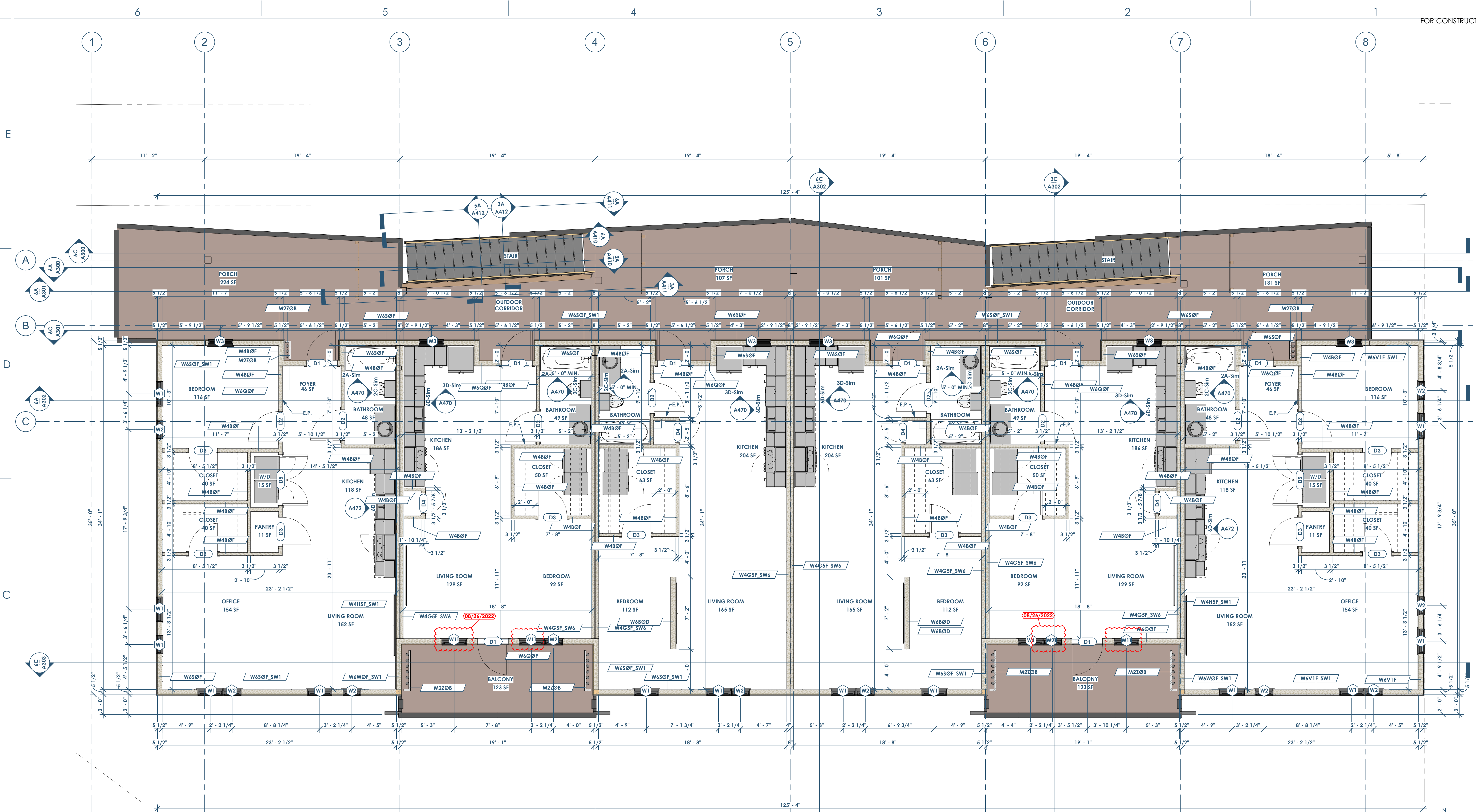
68 A103 FLOOR PLAN - 3RD FLOOR 1/4" = 1'-0"
