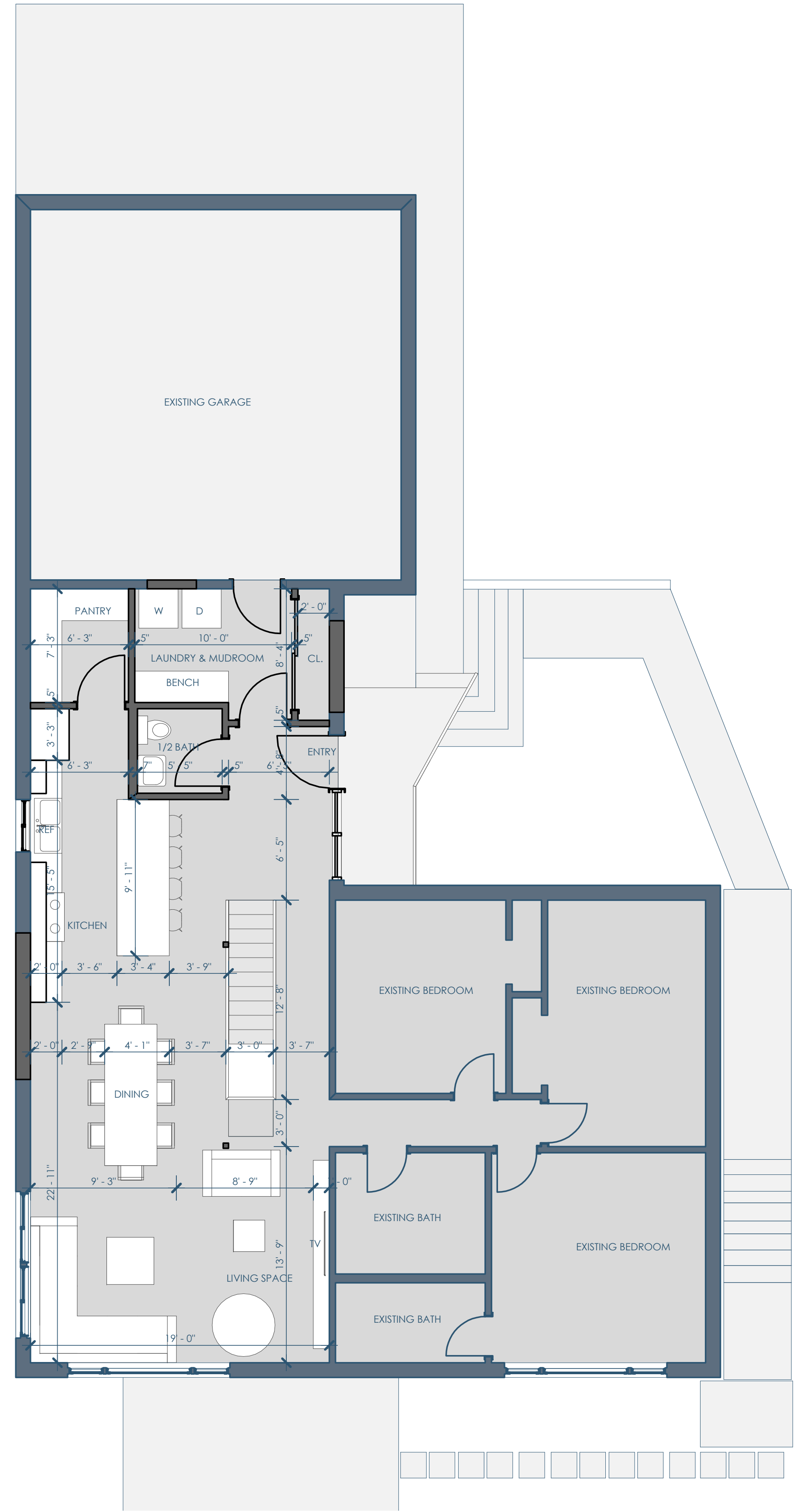
2A/A000 OPTION 2 - FLOOR PLAN 3/16"=1'-0"
