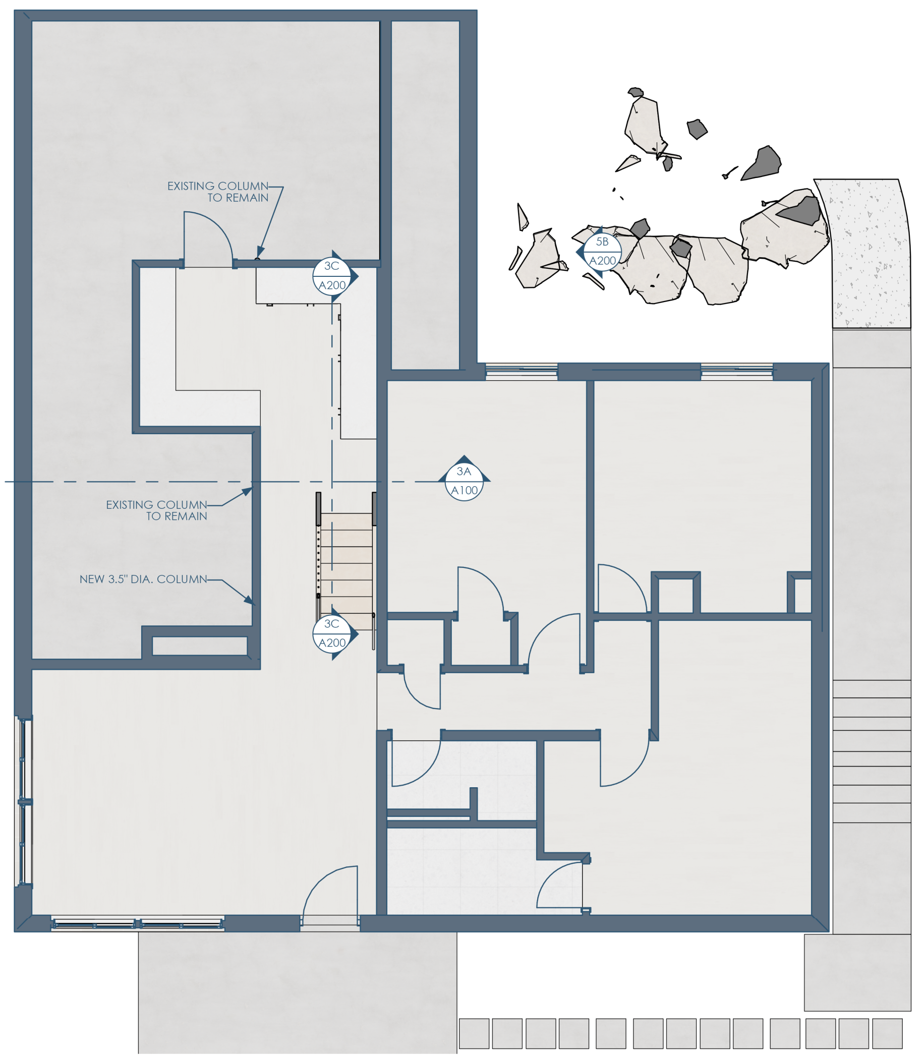
2B/A100 FLOOR PLAN - BASEMENT 3/16"=1'-0"
