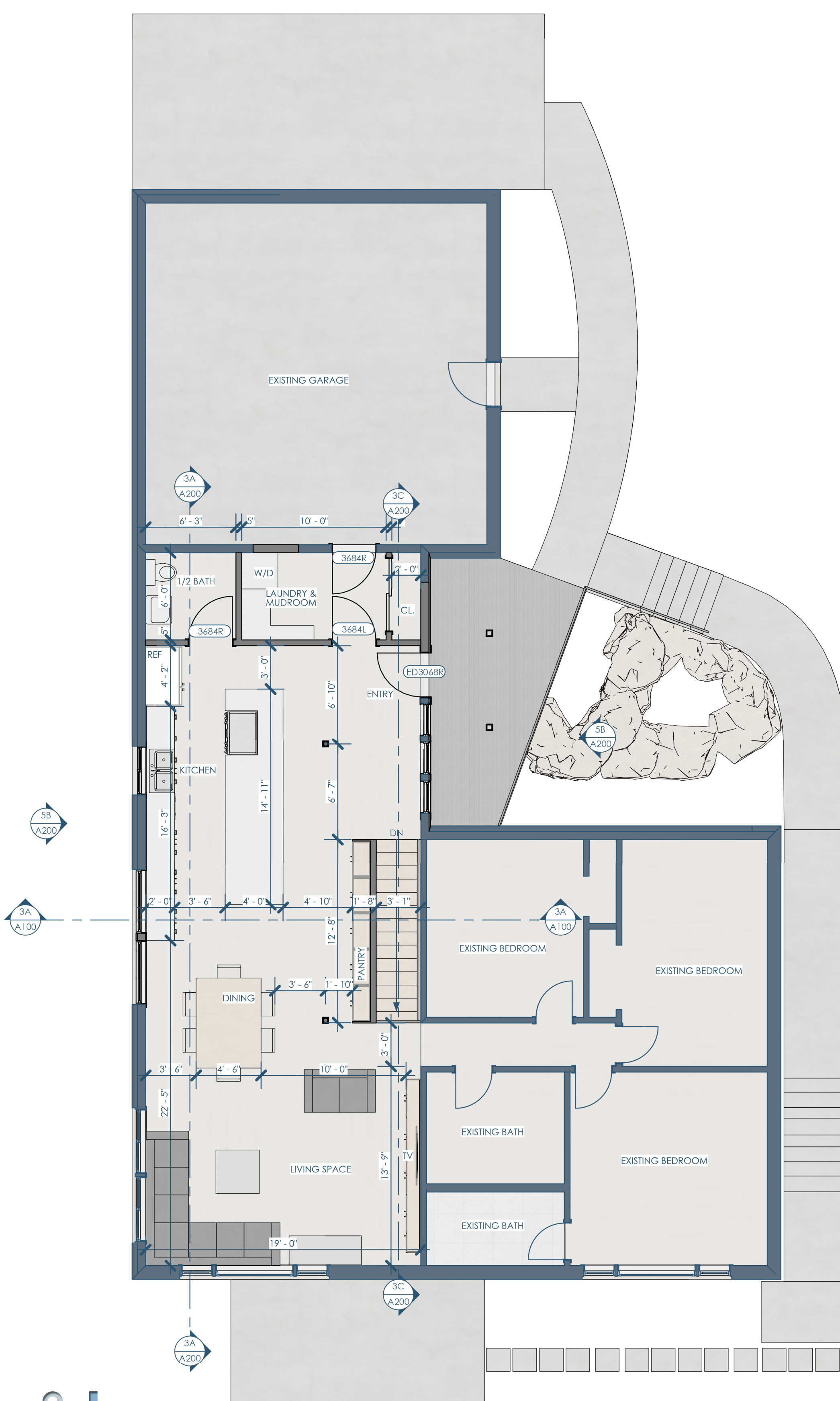
5A/A100 FLOOR PLAN - 1ST FLOOR 3/16"=1'-0"
