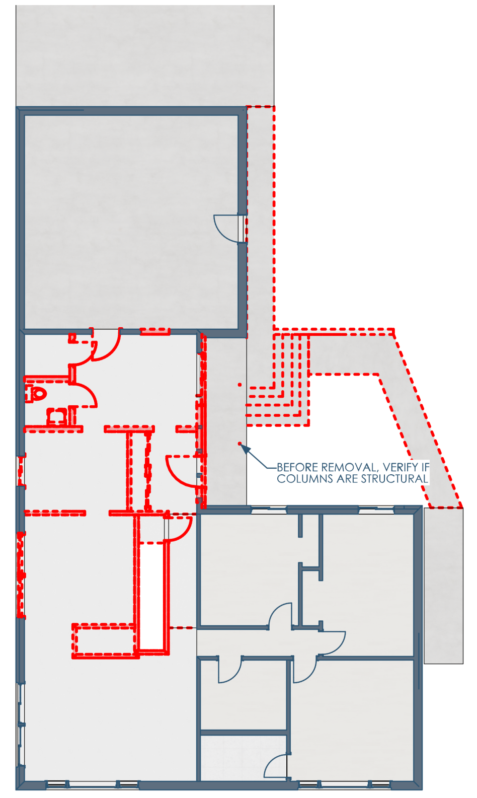
3B/A100 DEMO PLAN - 1ST FLOOR 3/32"=1'-0"
