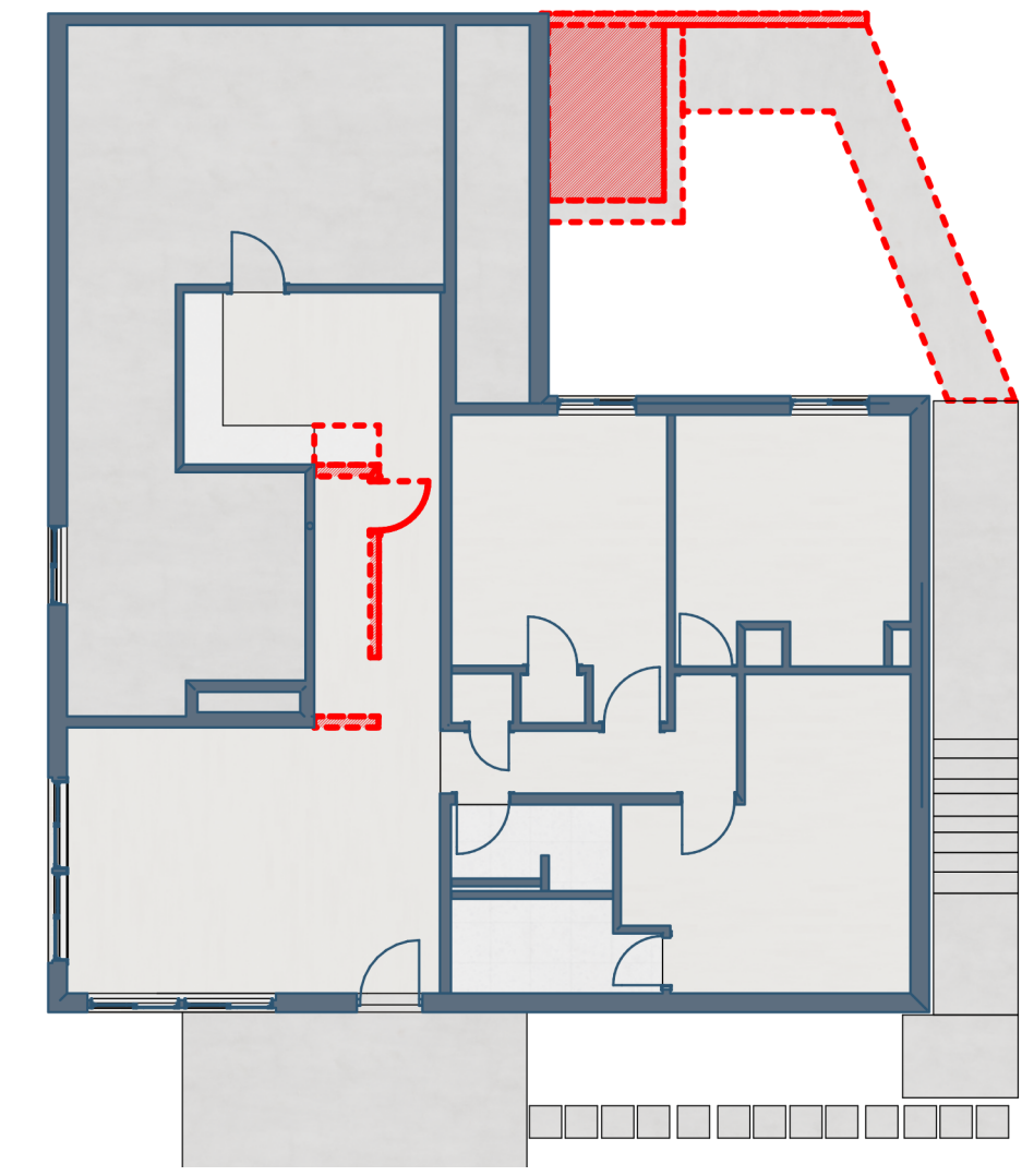
2A/A100 DEMO PLAN - BASEMENT 3/32"=1'-0"
