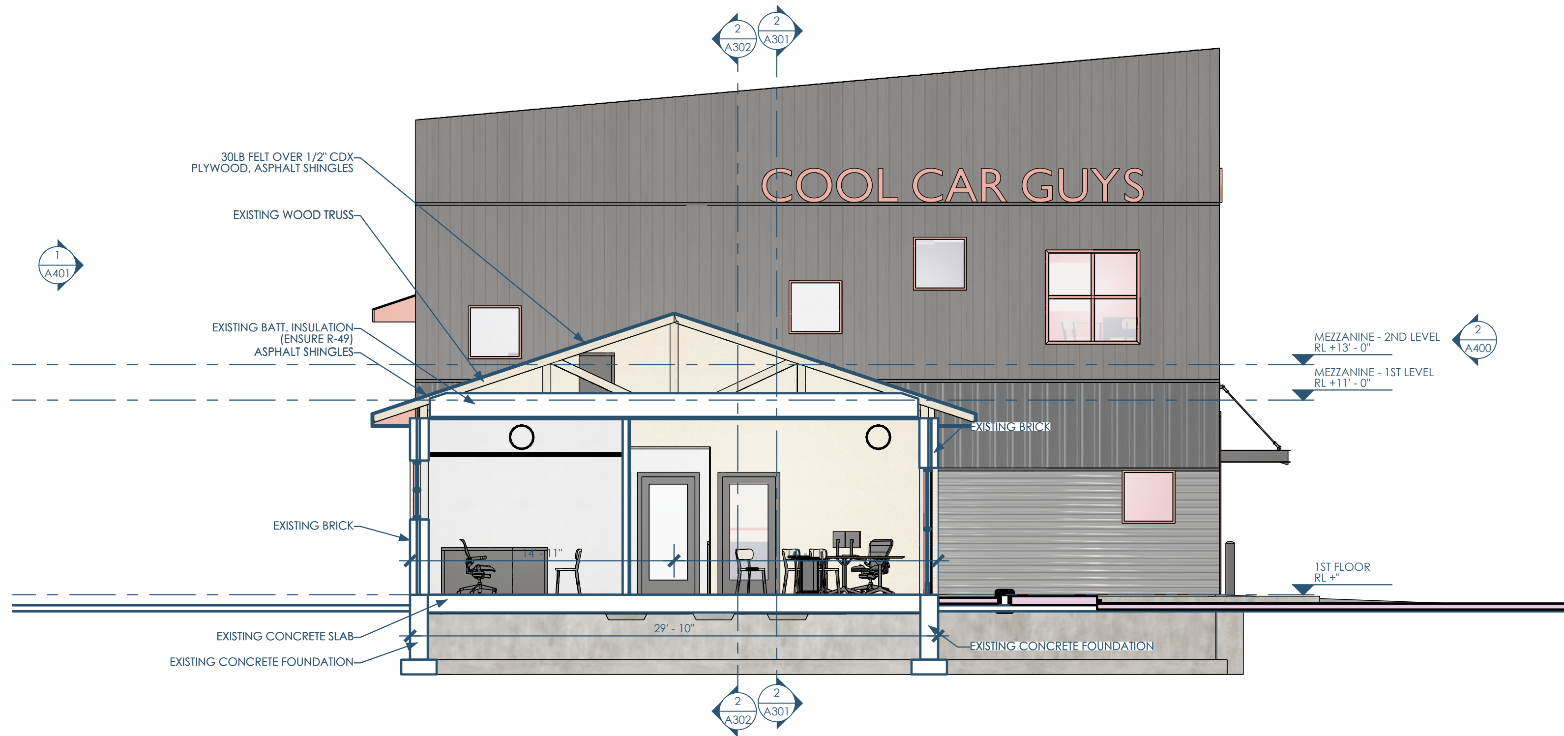
2/A303 SECTION - NS - WEST - AT EX. LOBBY 3/16"=1'-0"
