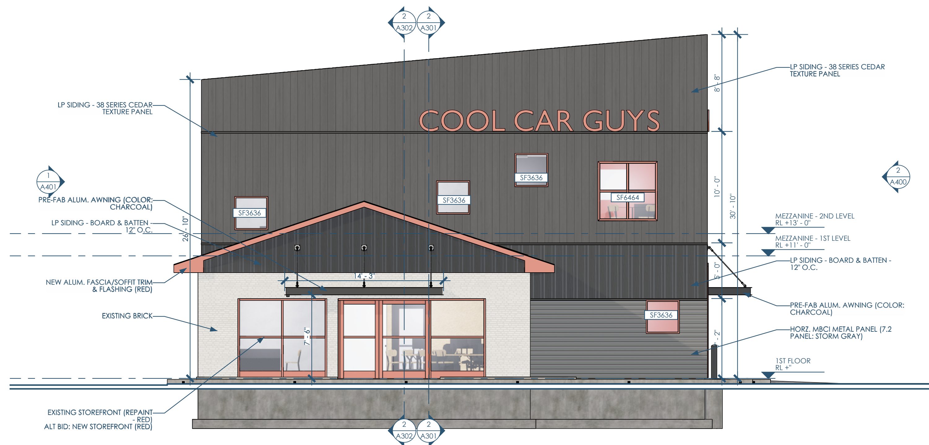
1/A400 ELEVATION - EAST - AT CENTER AVE 3/16"=1'-0"
