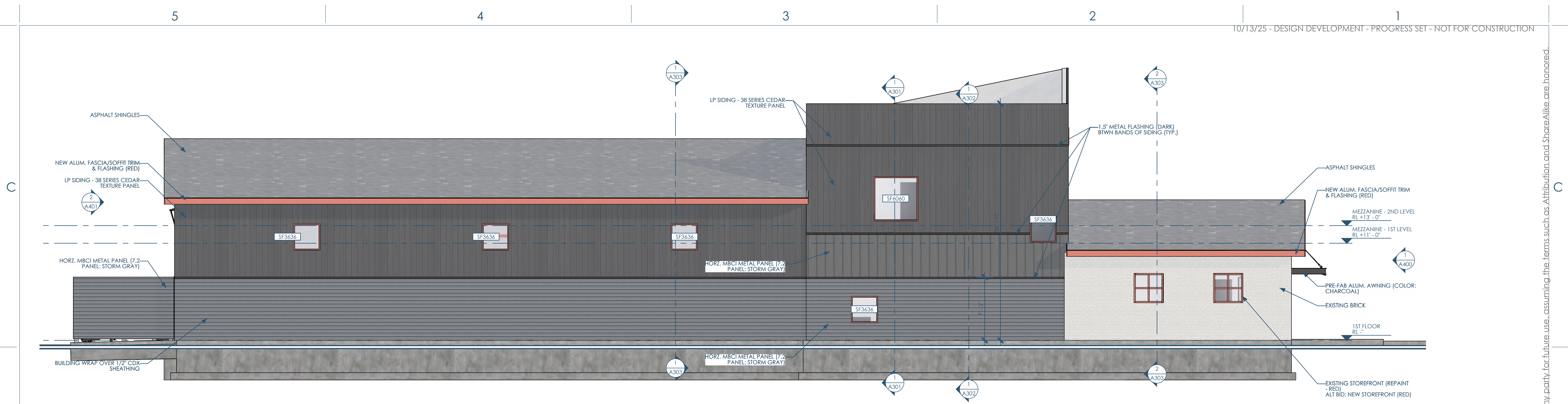
1/A401 ELEVATION - SOUTH 3/16"=1'-0"
