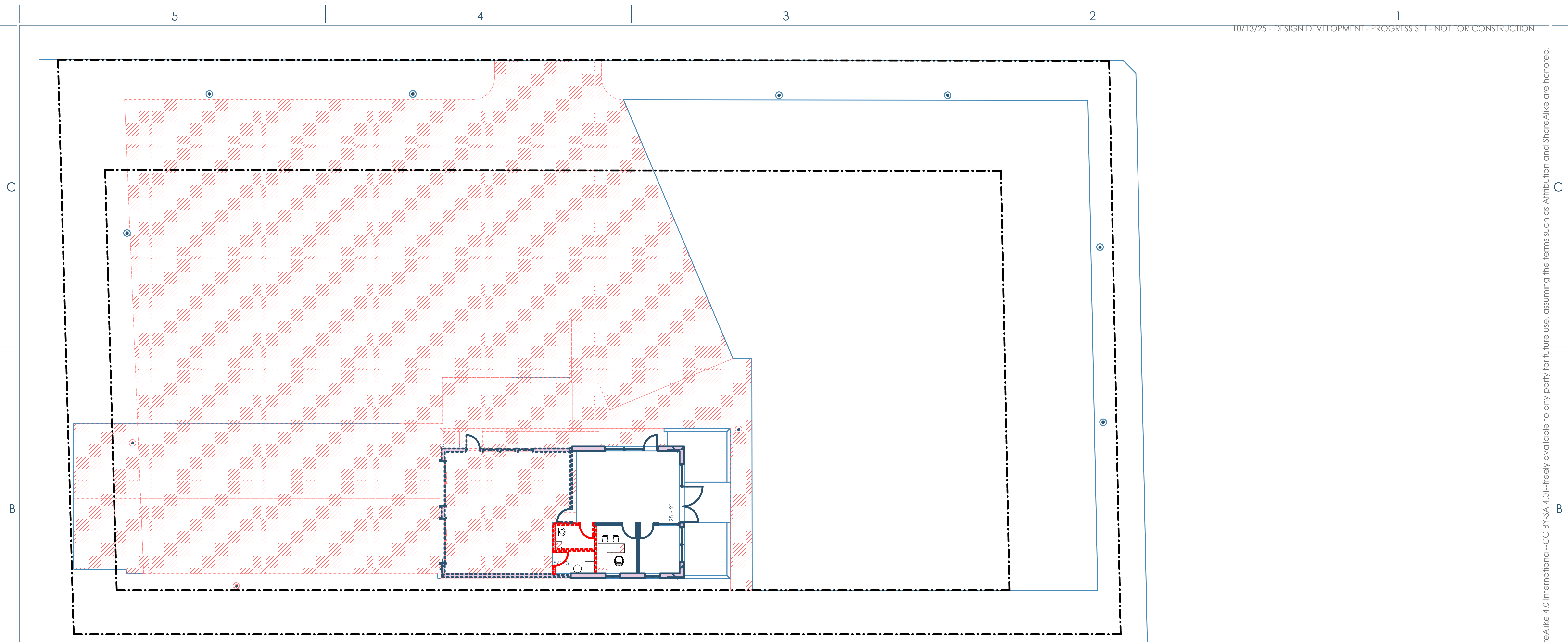
1/A050 PHASE 1 - DEMOLITION PLAN 3/32"=1'-0"
