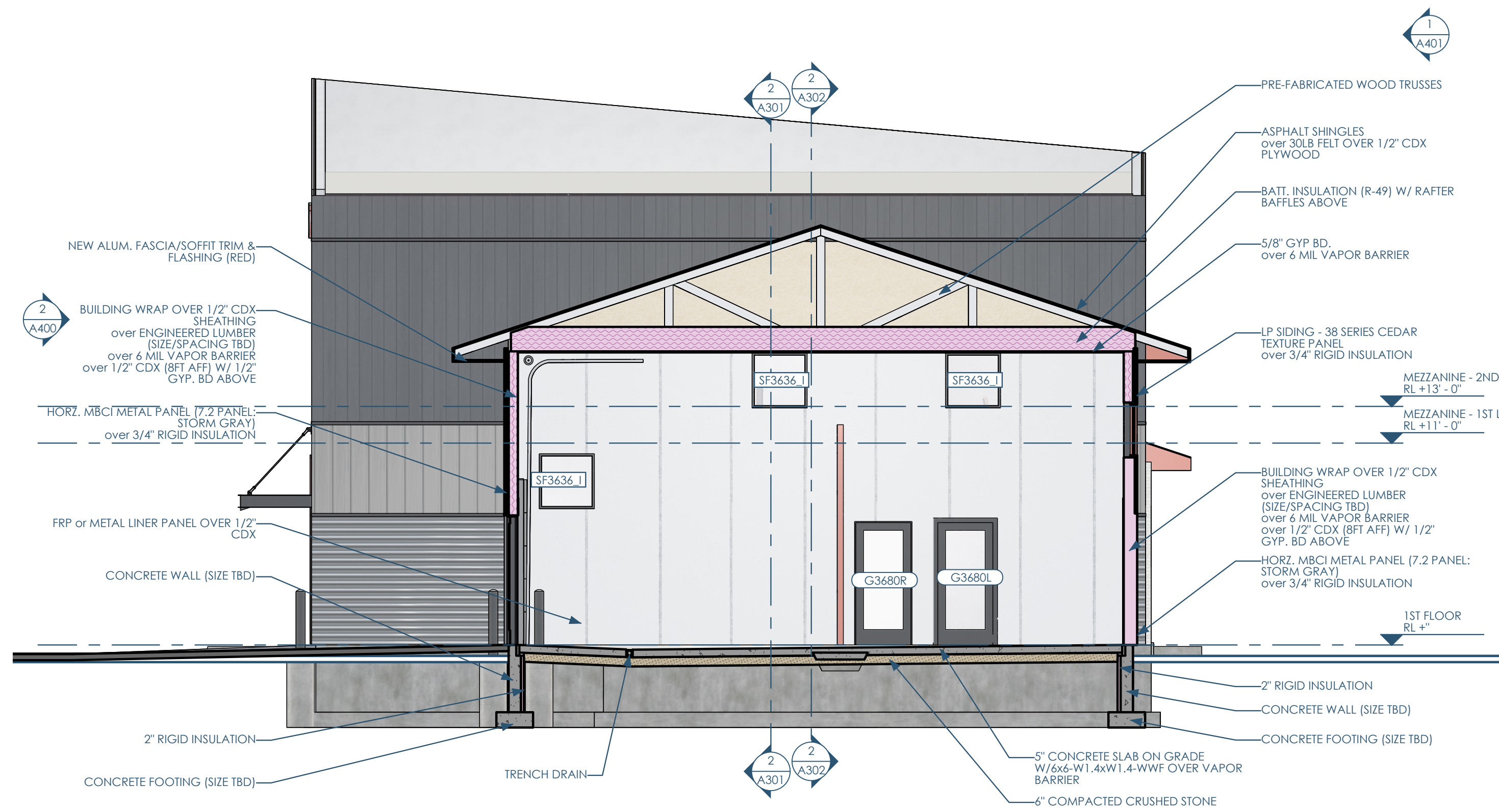
1/A303 SECTION - NS - EAST - AT SERVICE BAY 3/16"=1'-0"
