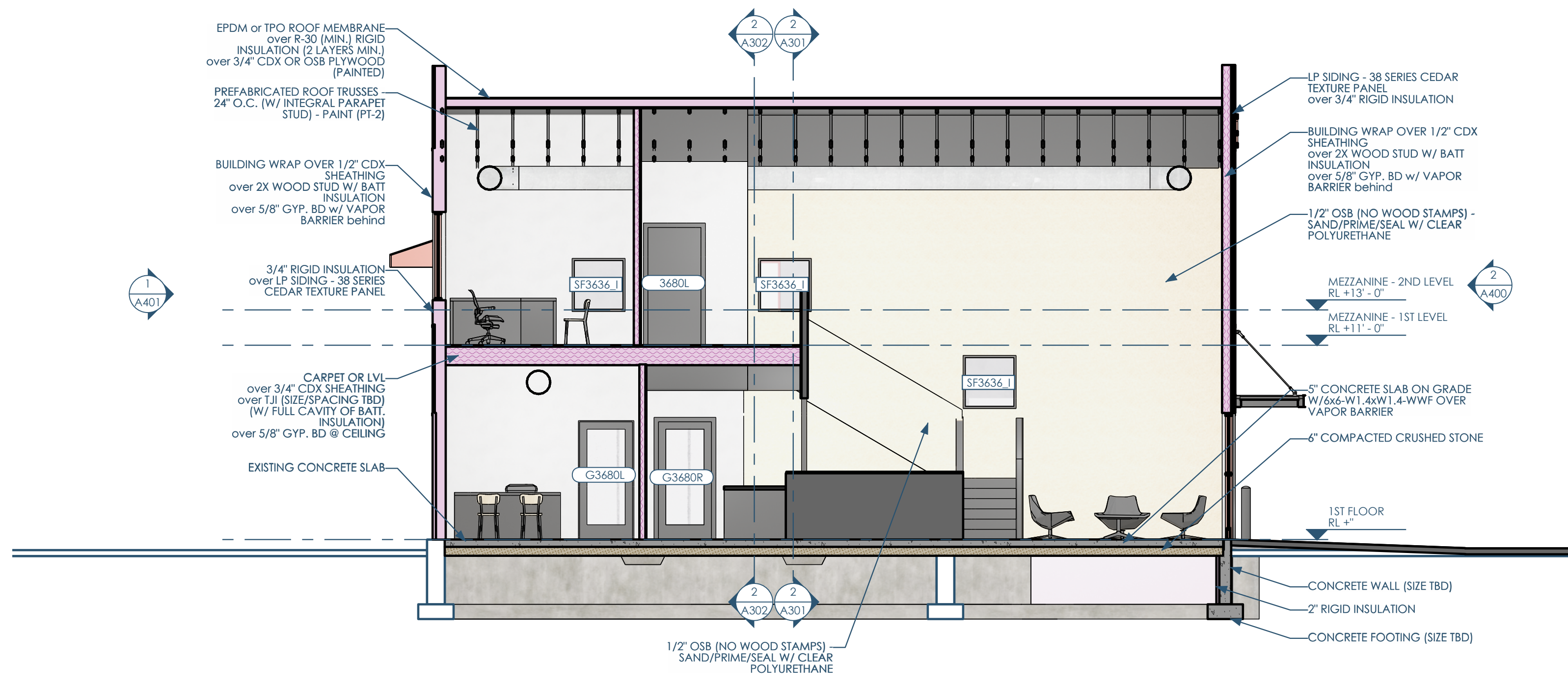
1/A301 SECTION - NS - WEST - AT LOBBY 3/16"=1'-0"
