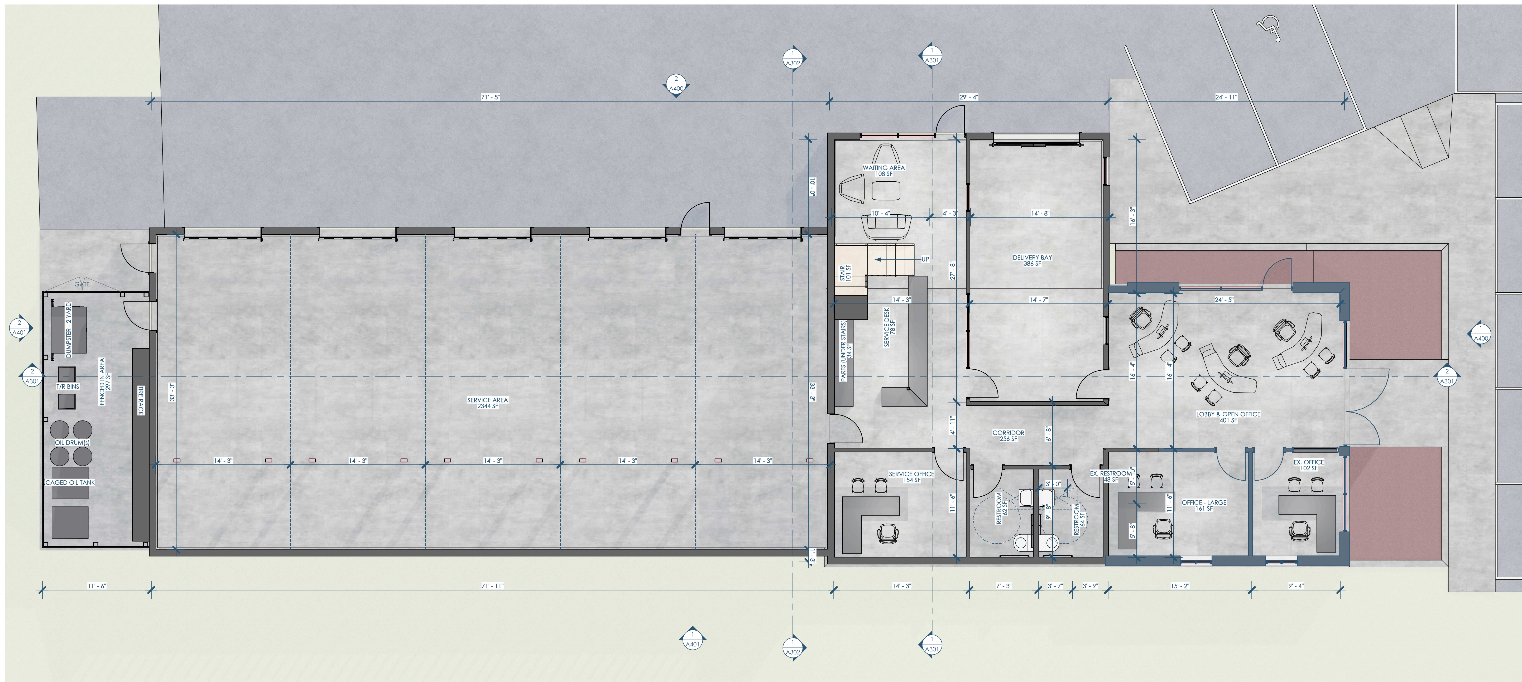
1/A101_2 PHASE 2 - 1ST FLOOR 3/16"=1'-0"
