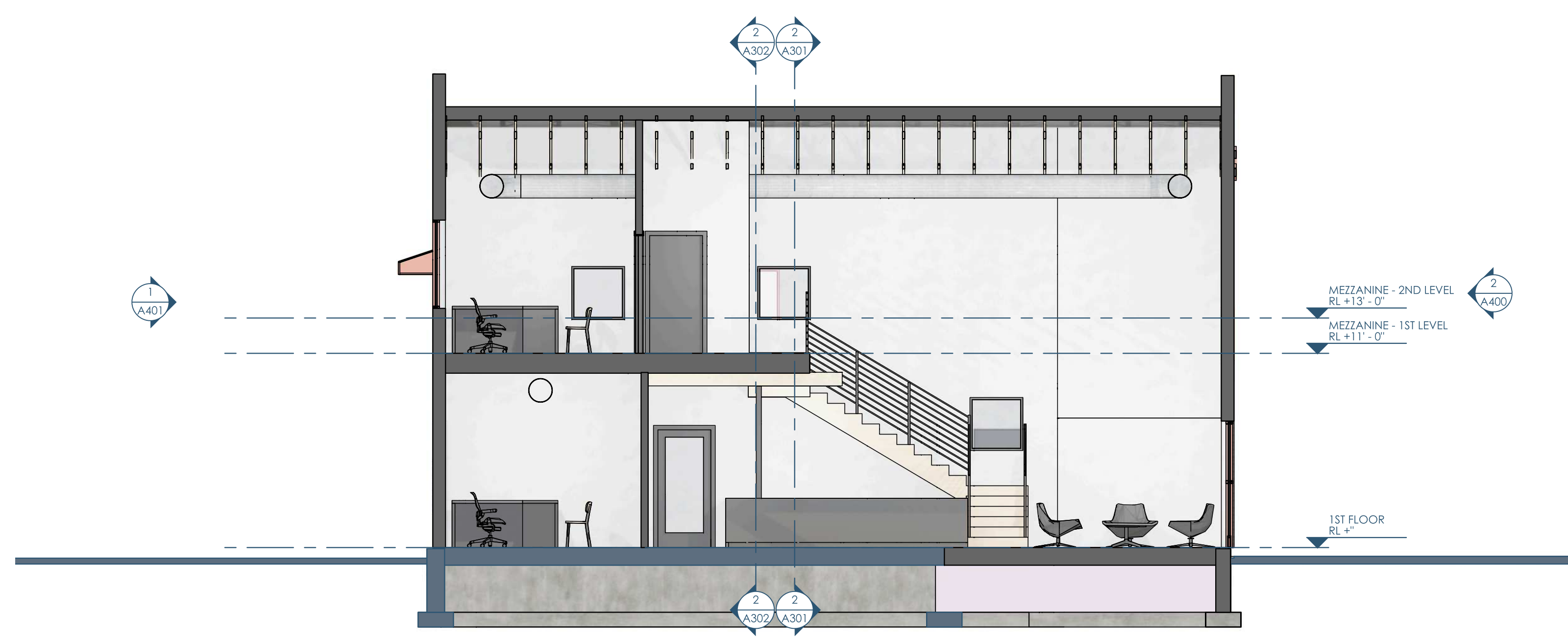
1/A301 SECTION - NS - WEST AT LOBBY 3/16"=1'-0"
