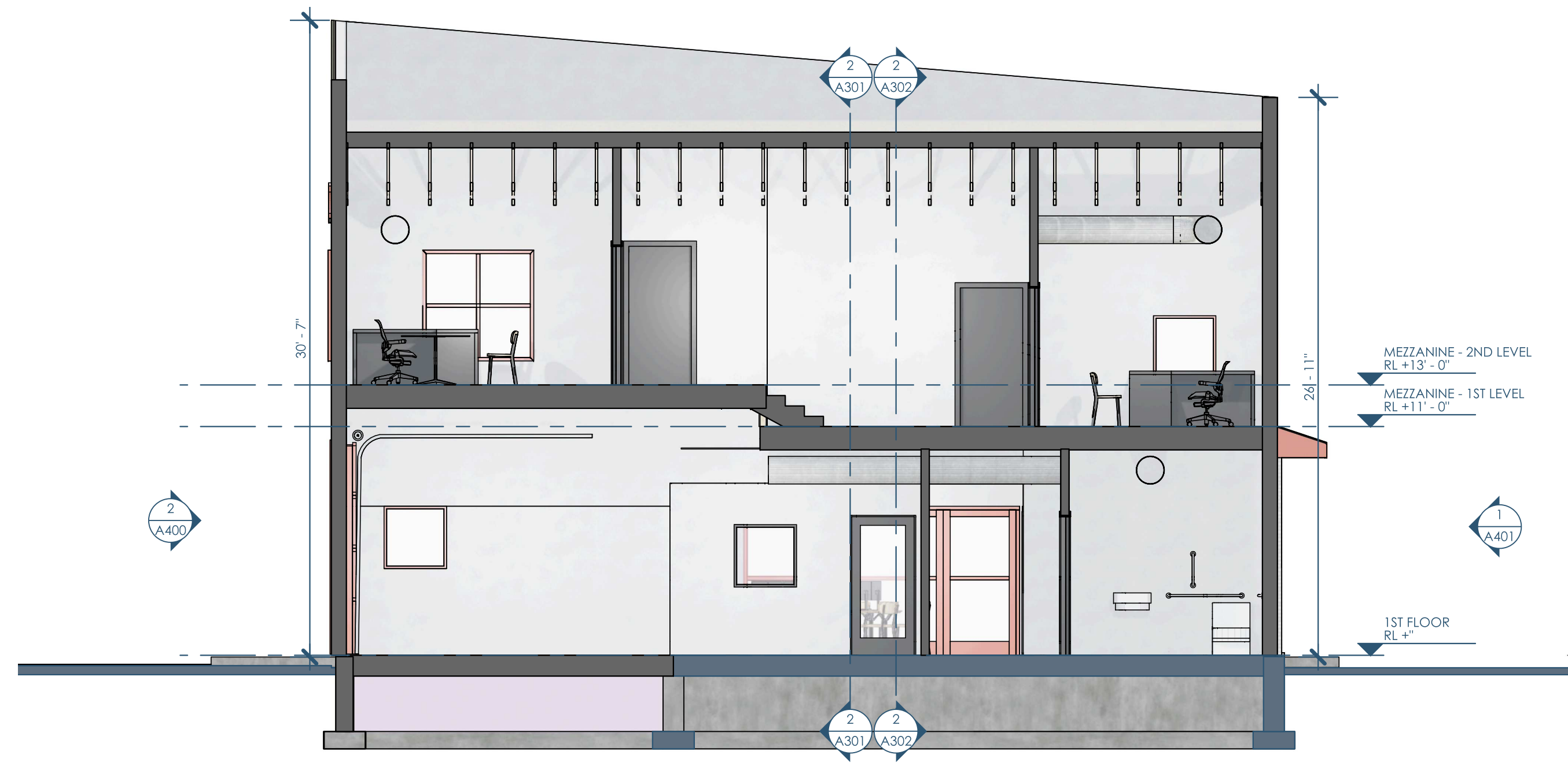
1/A302 SECTION - NS - EAST AT DROPOFF BAY 3/16"=1'-0"
