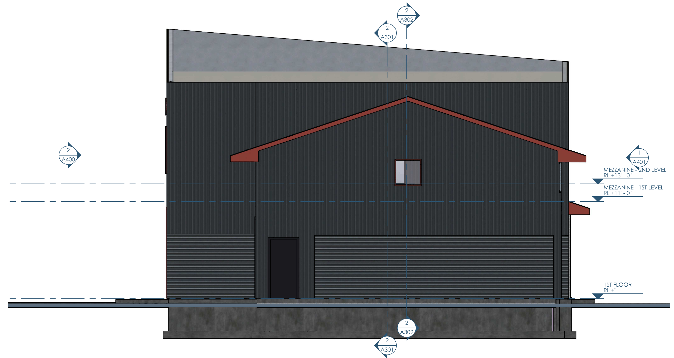
2/A401 ELEVATION - WEST 3/16"=1'-0"
