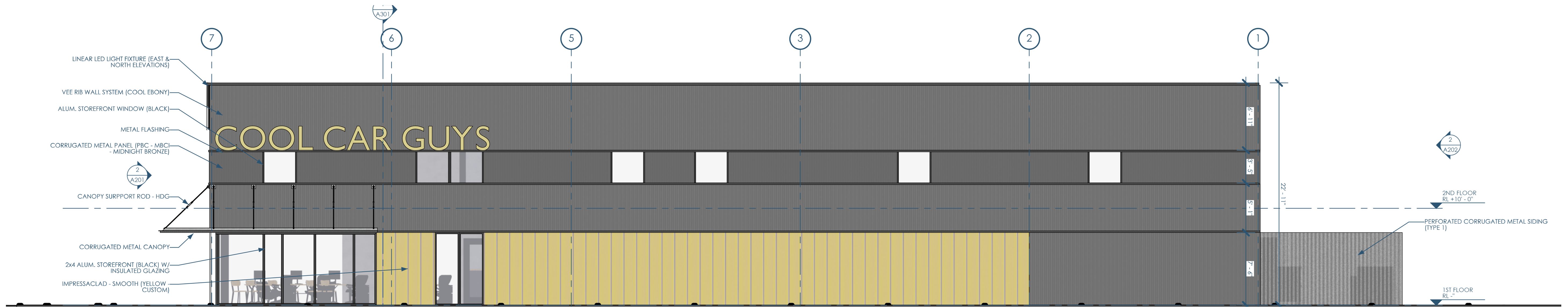
2/A201 ELEVATION - NORTH JOLIET ST. 3/16"=1'-0"
