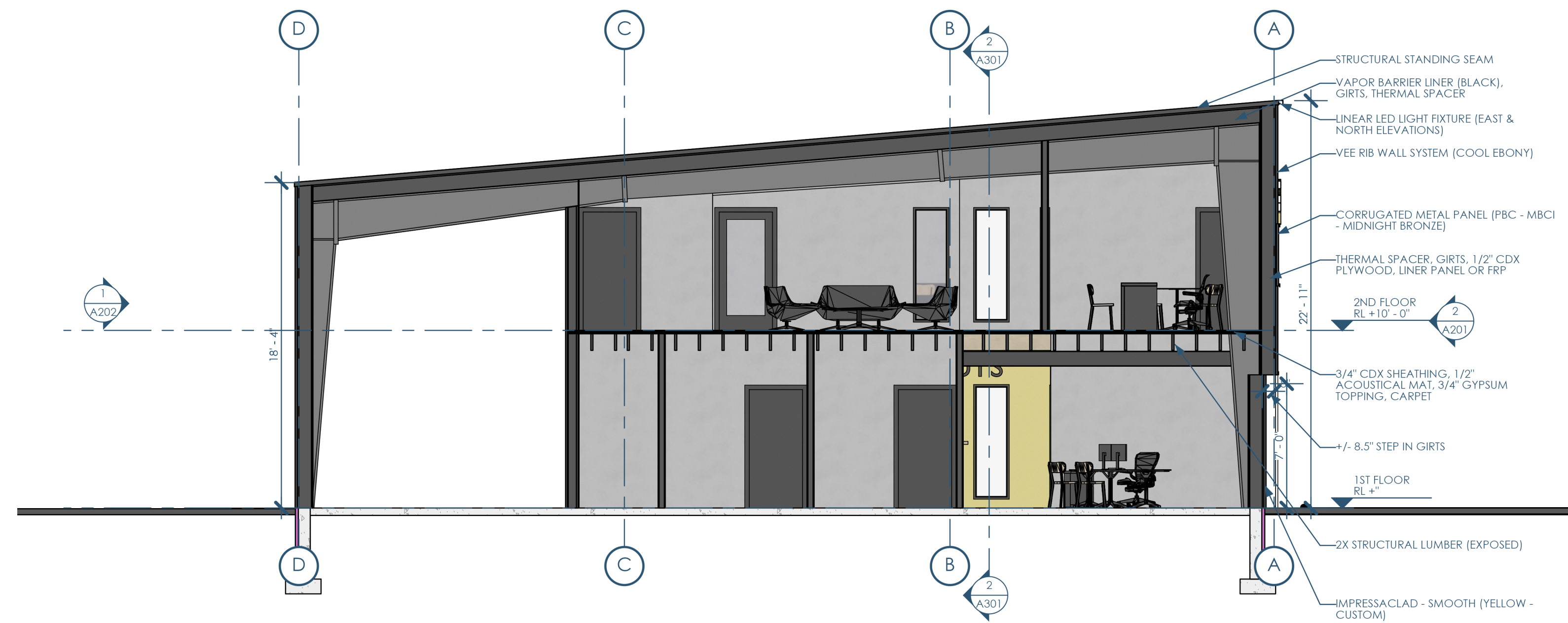
1/A301 SECTION - NS - WEST 3/16"=1'-0"
