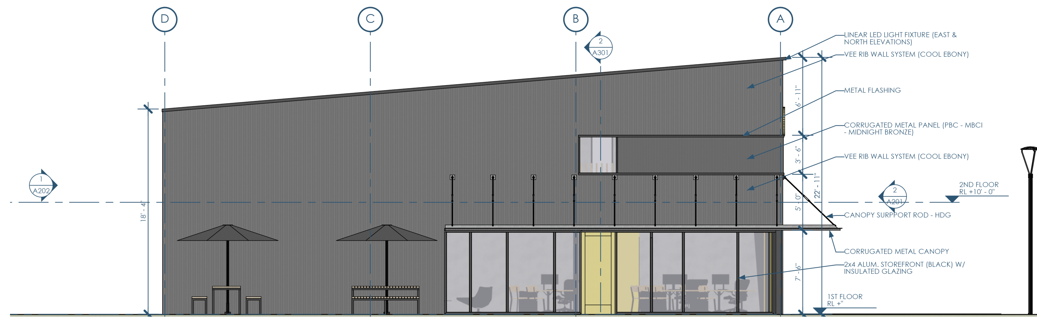
2/A201 ELEVATION - EAST CENTER AVE. 3/16"=1'-0"
