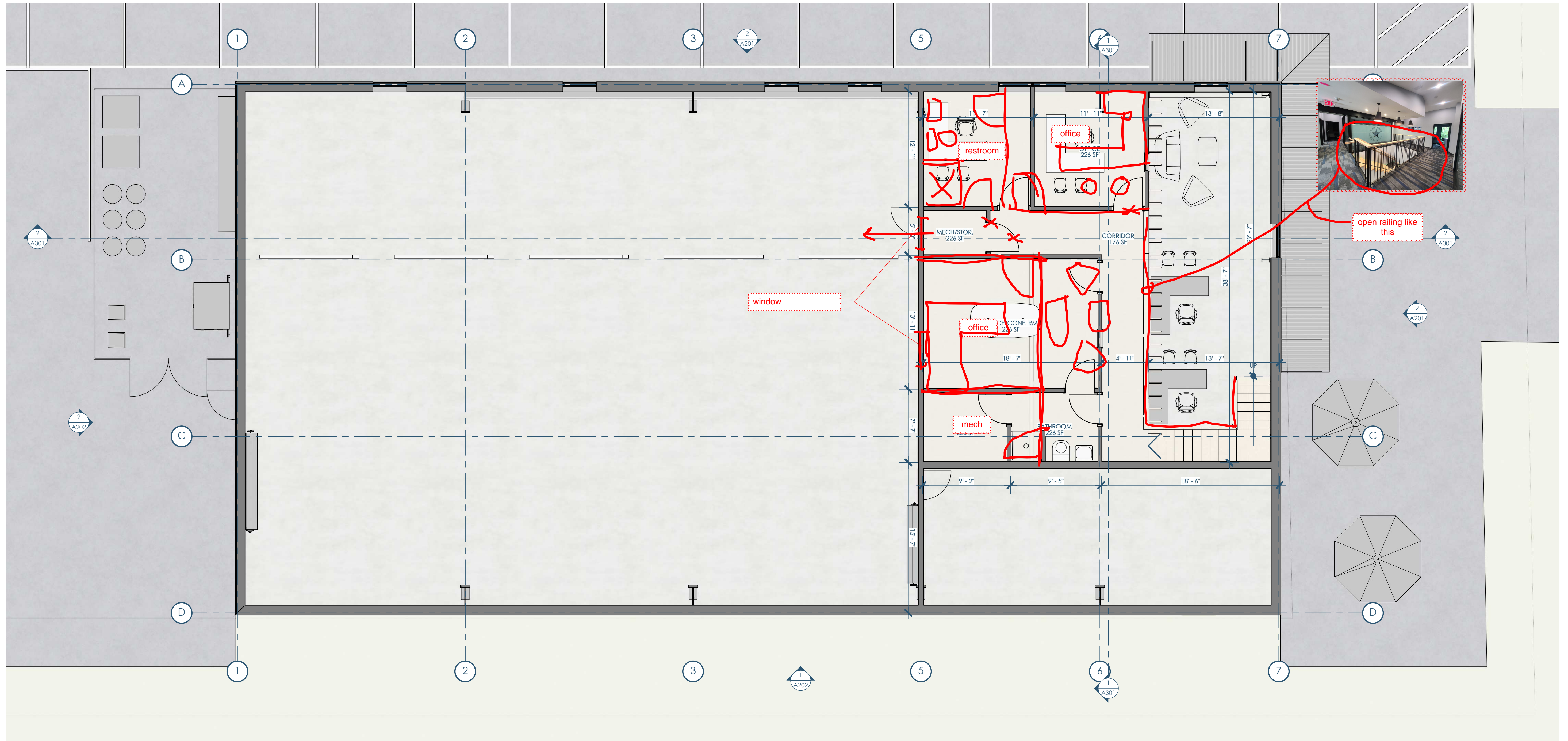
1/A102 FLOOR PLAN - MEZZ. 3/16"=1'-0"
