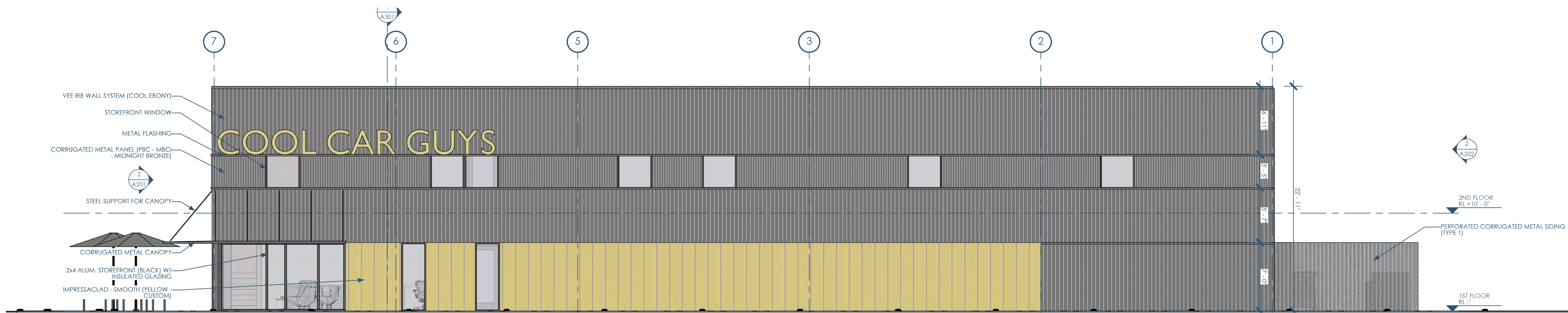
2/A201 ELEVATION - NORTH JOLIET ST. 3/16"=1'-0"
