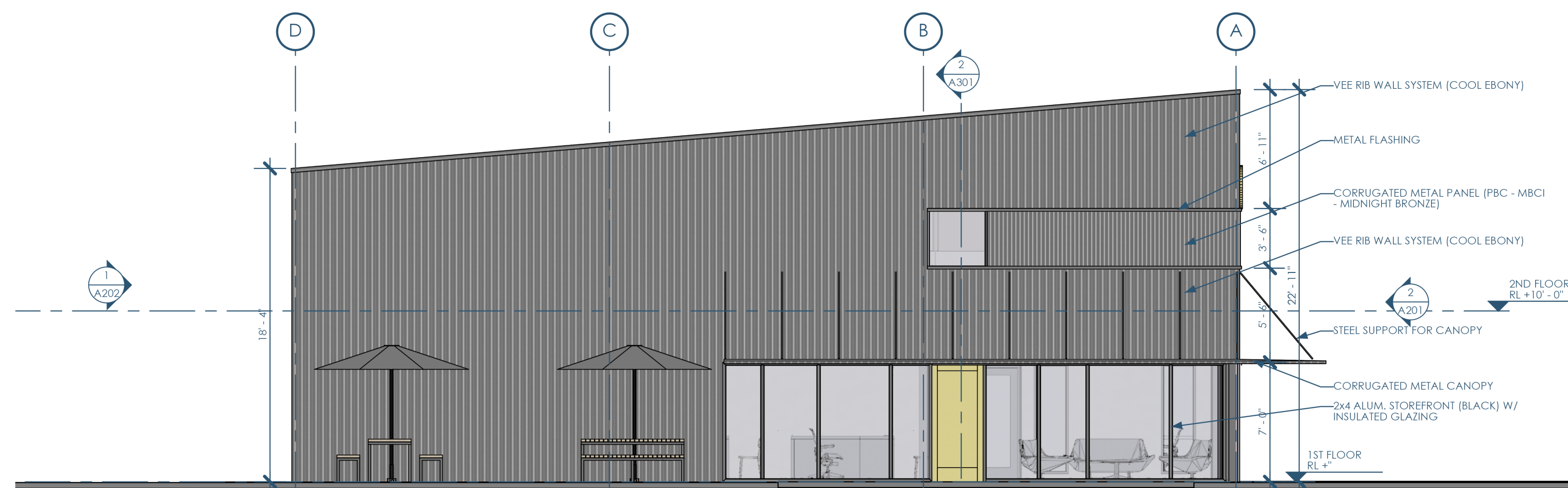
2/A201 ELEVATION - EAST CENTER AVE. 3/16"=1'-0"
