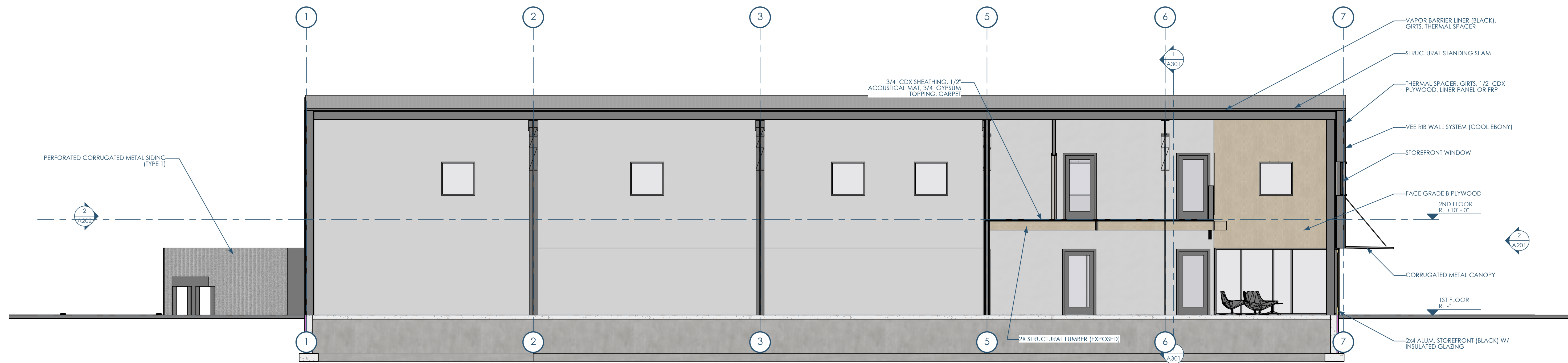
2/A301 SECTION NORTH 3/16"=1'-0"
