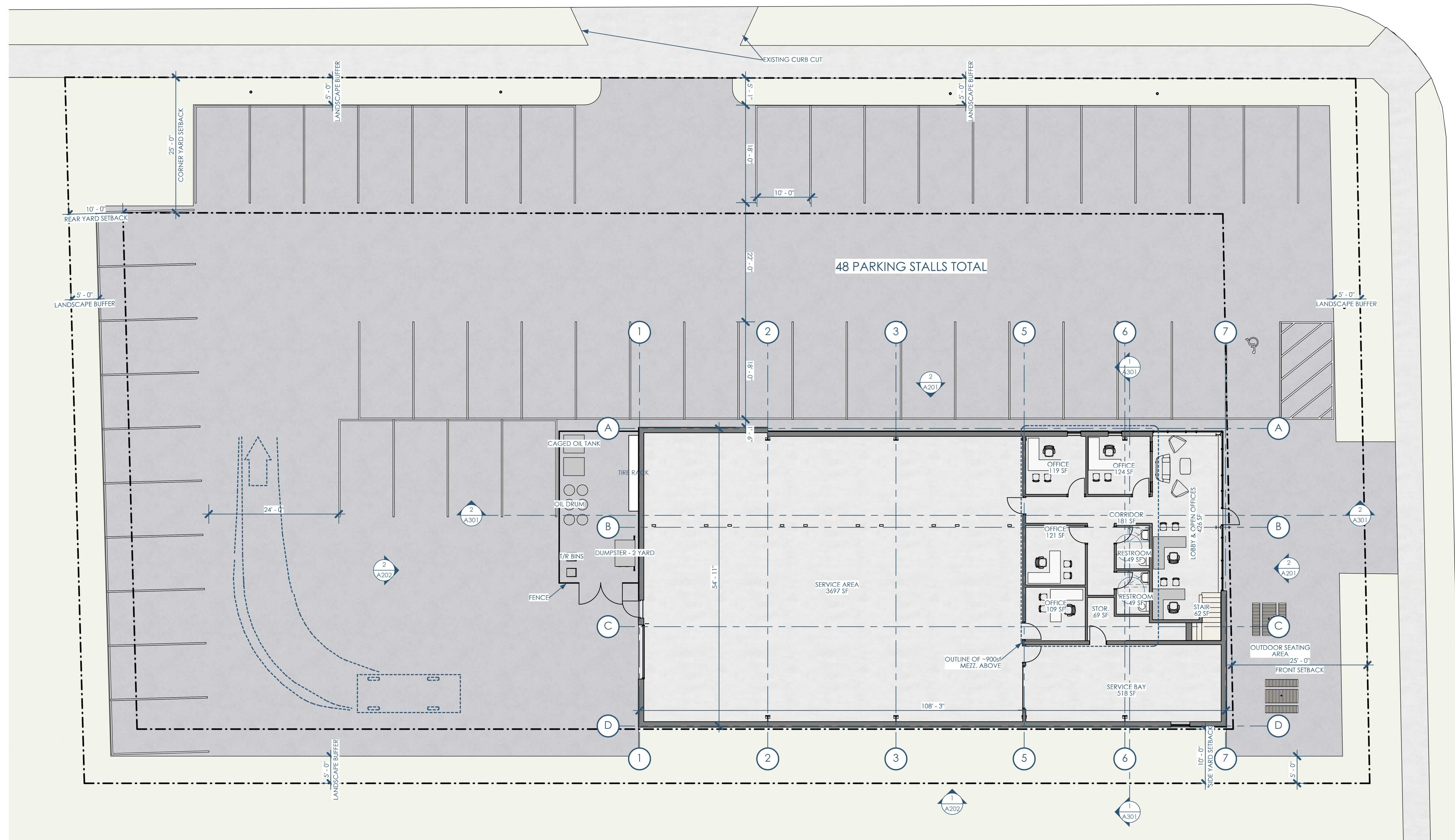
1/A100 SITE PLAN 1"=10'
