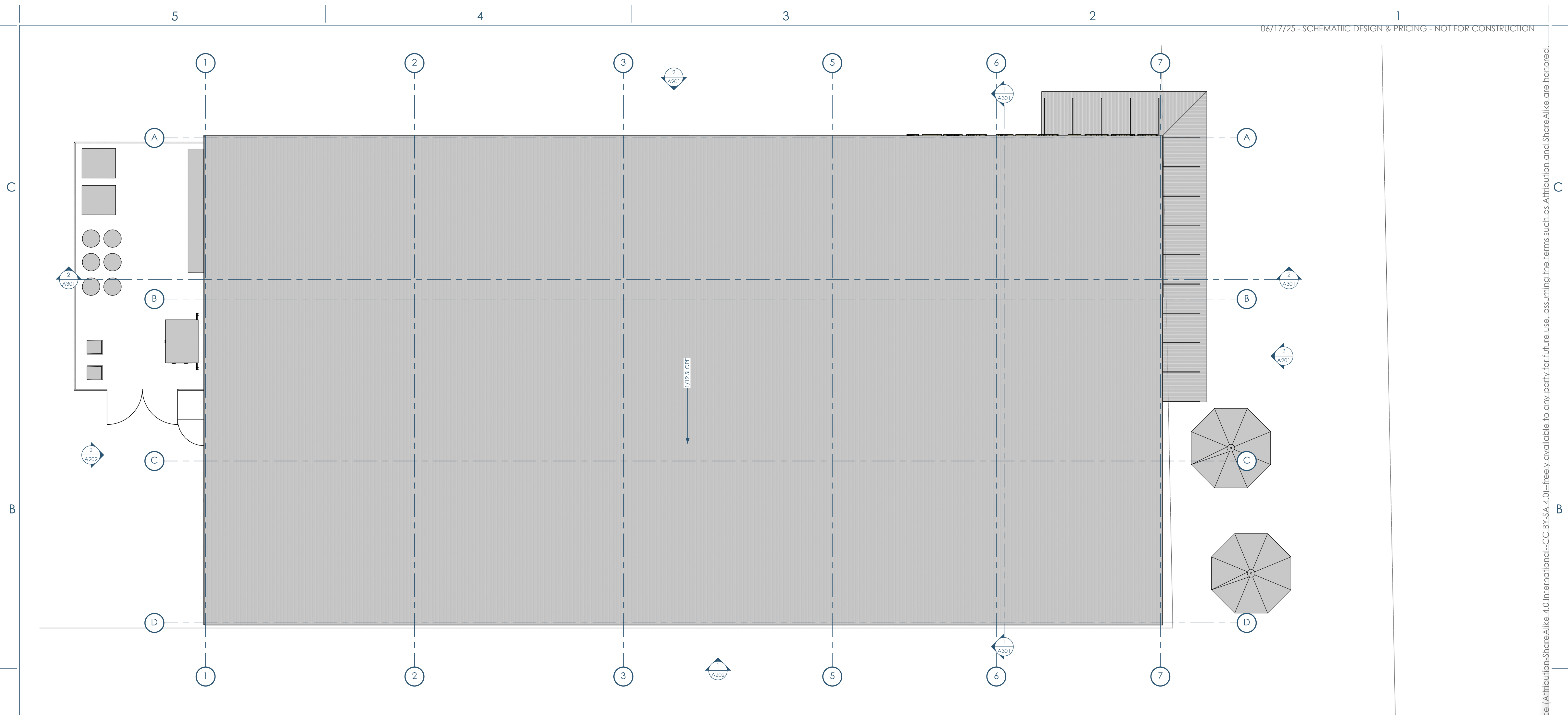
1/A103 FLOOR PLAN - ROOF 3/16"=1'-0"
