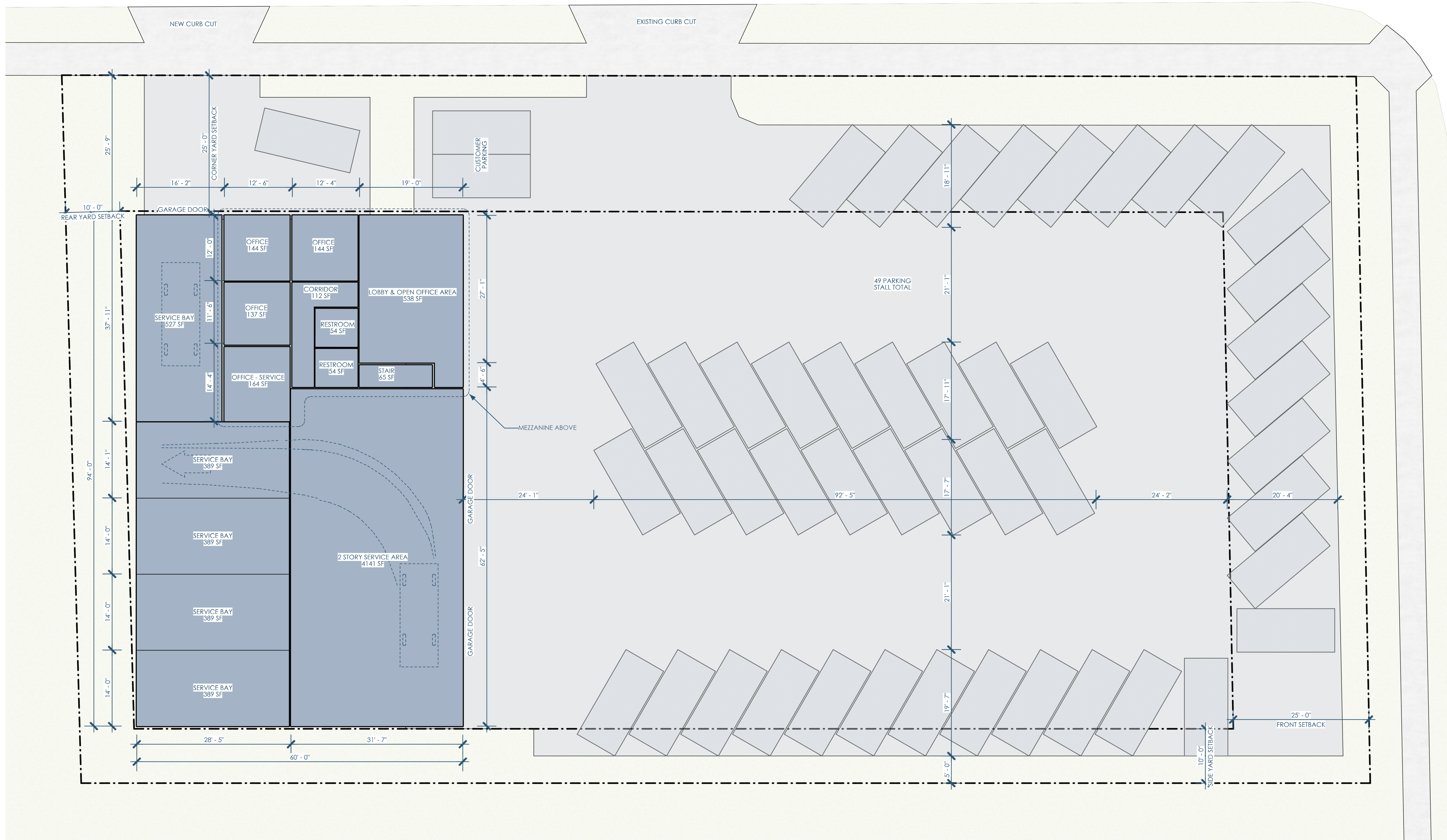
1/07-1 LAYOUT OPTION 7 - 1ST FLOOR 1"=10'
