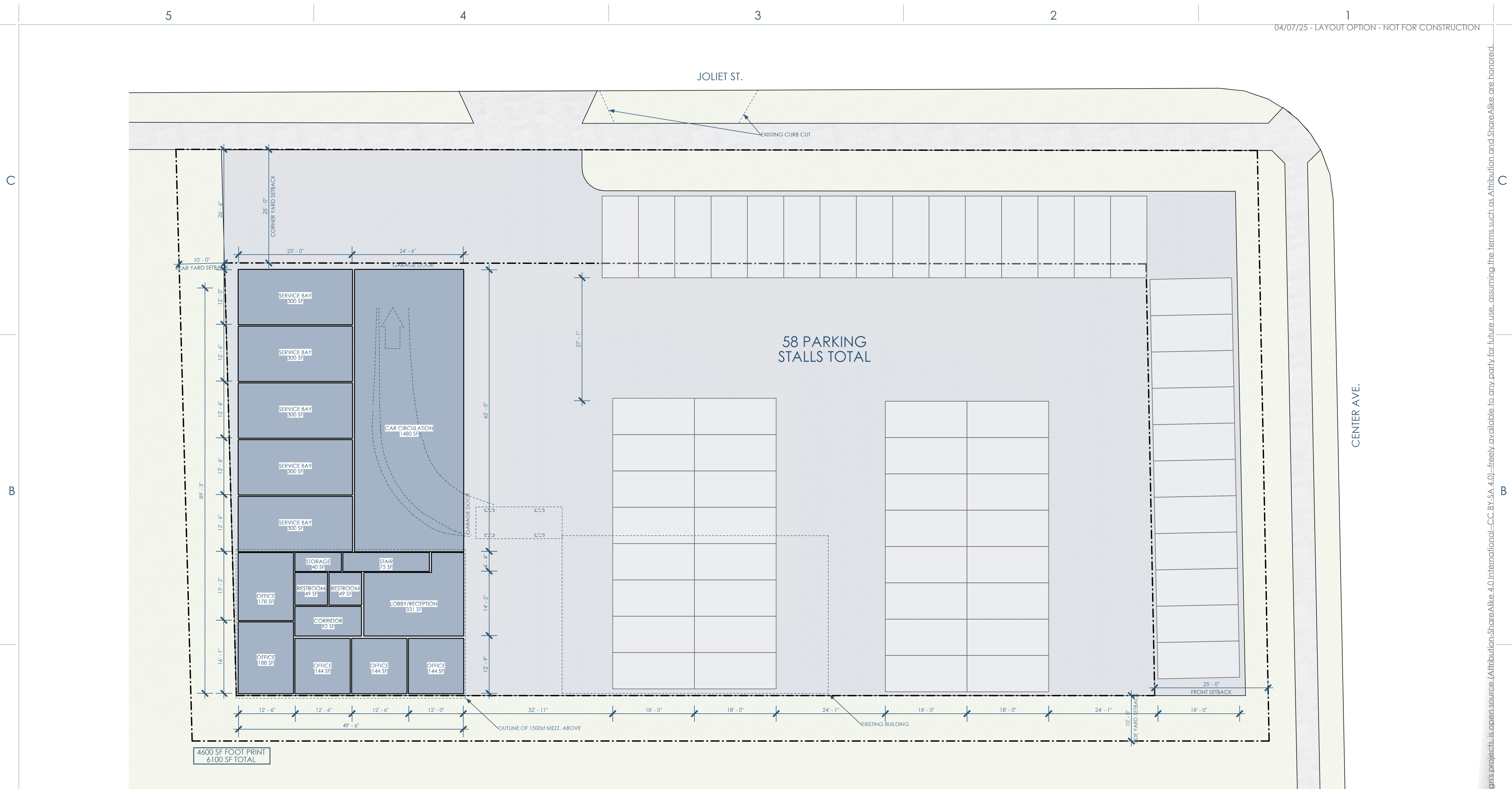
1/01 LAYOUT OPTION 1 1"=10'
