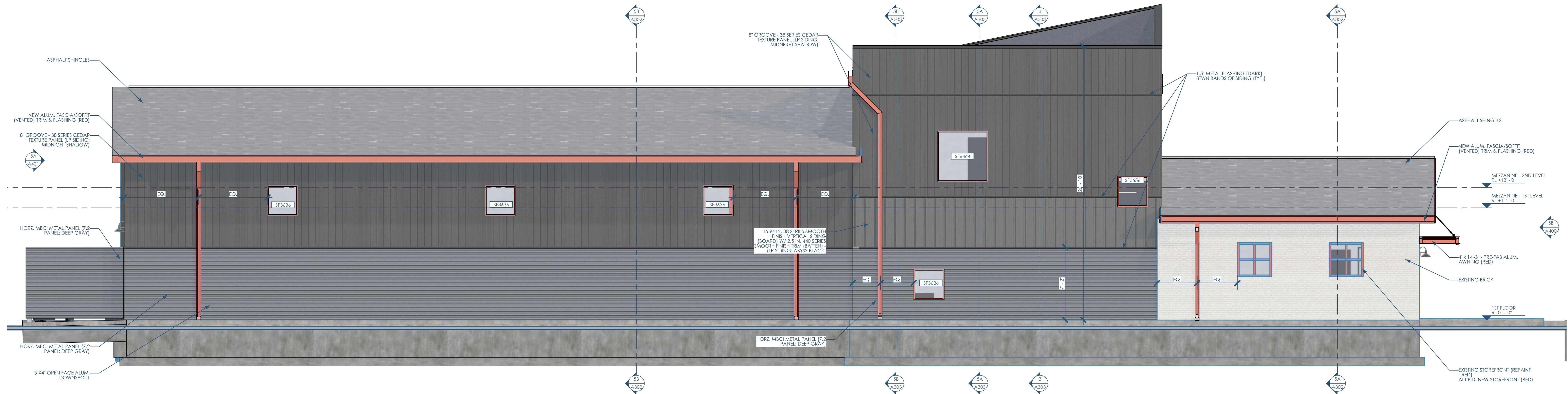
5B/A401 ELEVATION - SOUTH 1/4"=1'-0"
