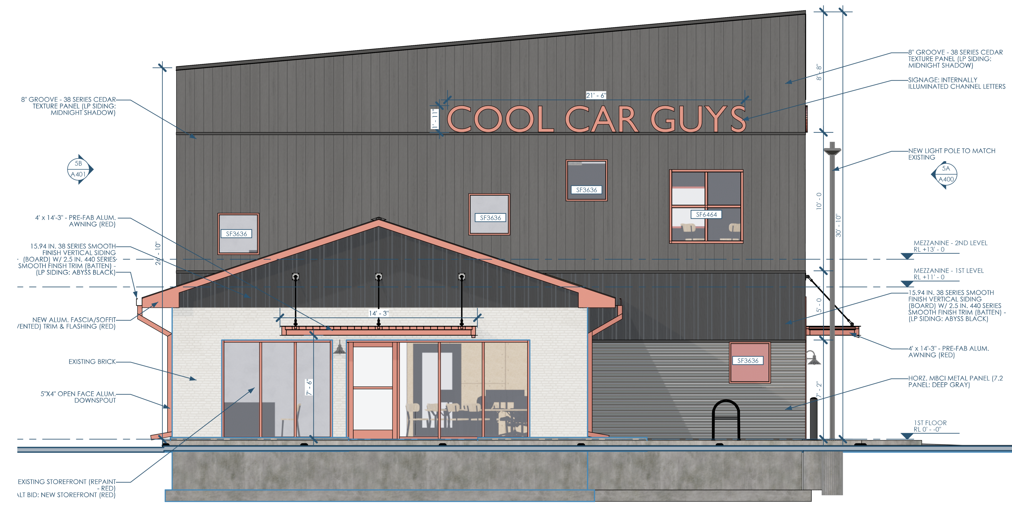
5B/A400 ELEVATION - EAST - AT CENTER AVE 1/4"=1'-0"
