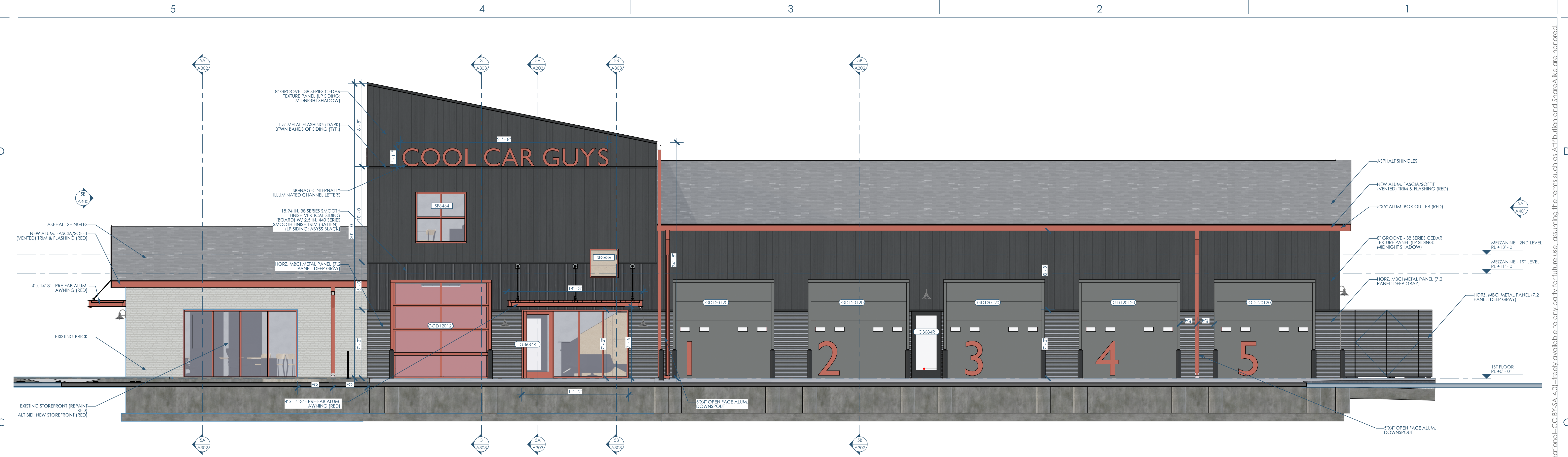
5A/A400 ELEVATION - NORTH - AT JOLIET ST 1/4"=1'-0"
