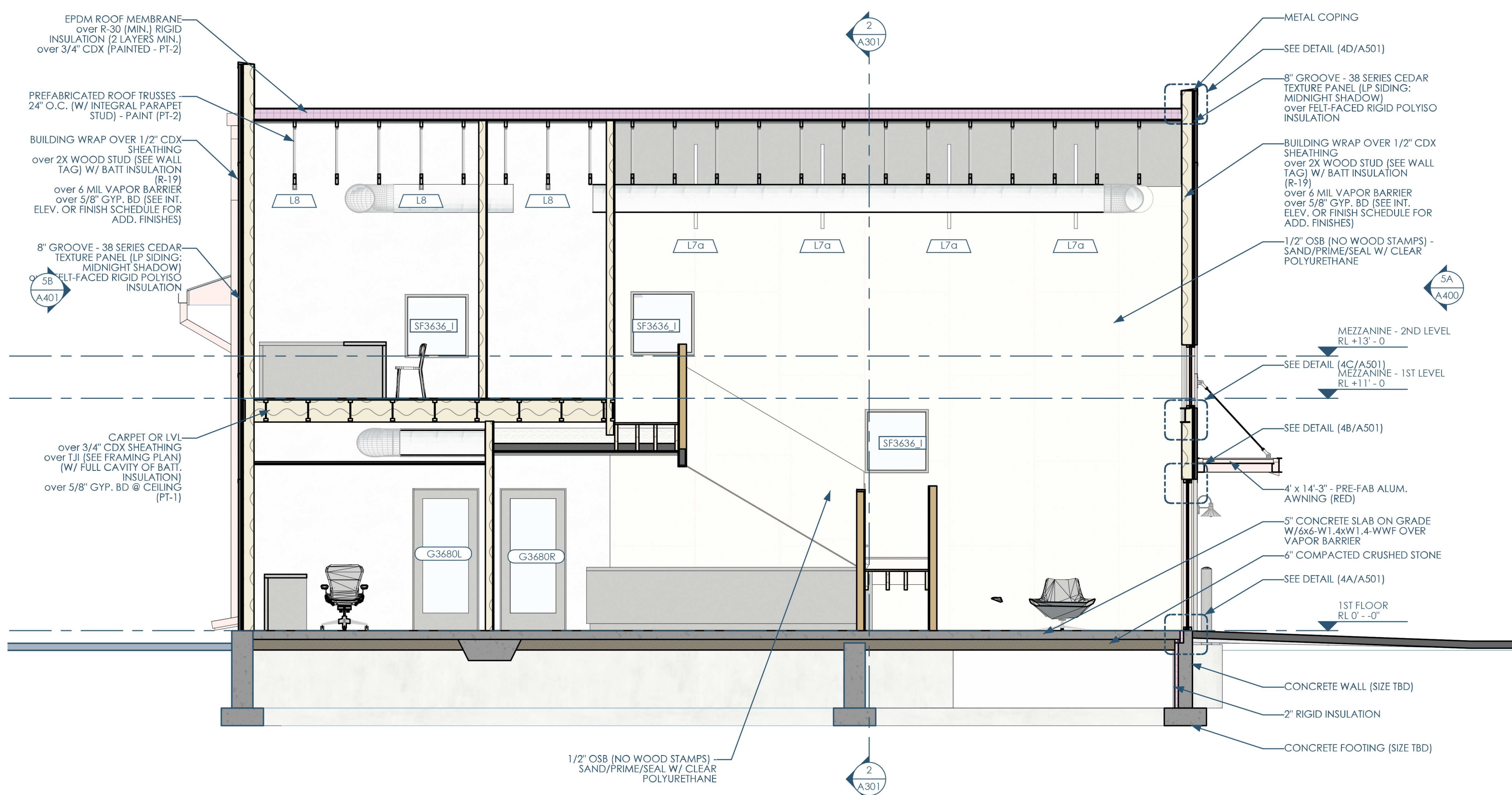
SB/A303 SECTION - NS - WEST - AT LOBBY AND STAIRS 1/4"=1'-0"
