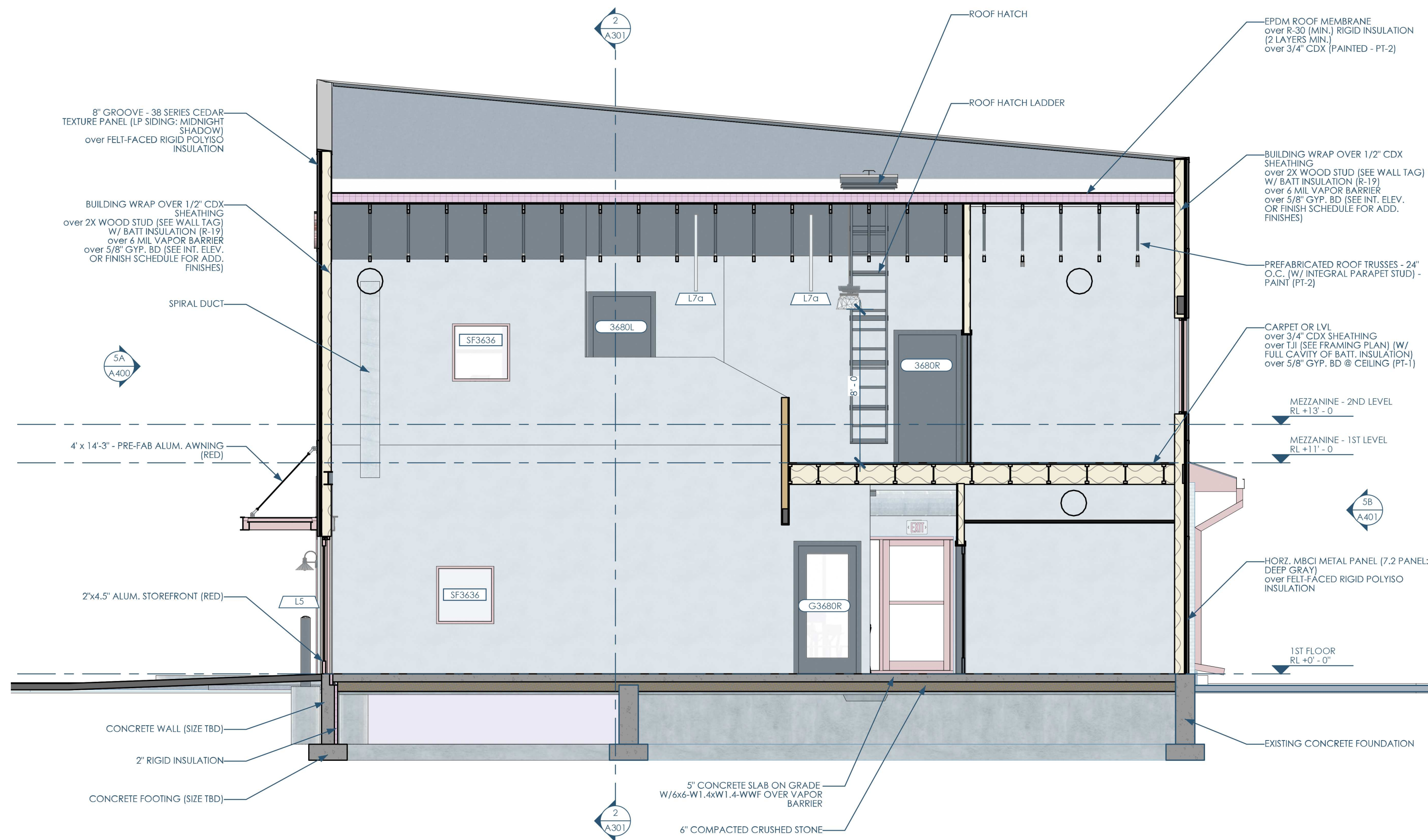
5A/A303 SECTION - NS - EAST - AT LOBBY 1/4"=1'-0"
