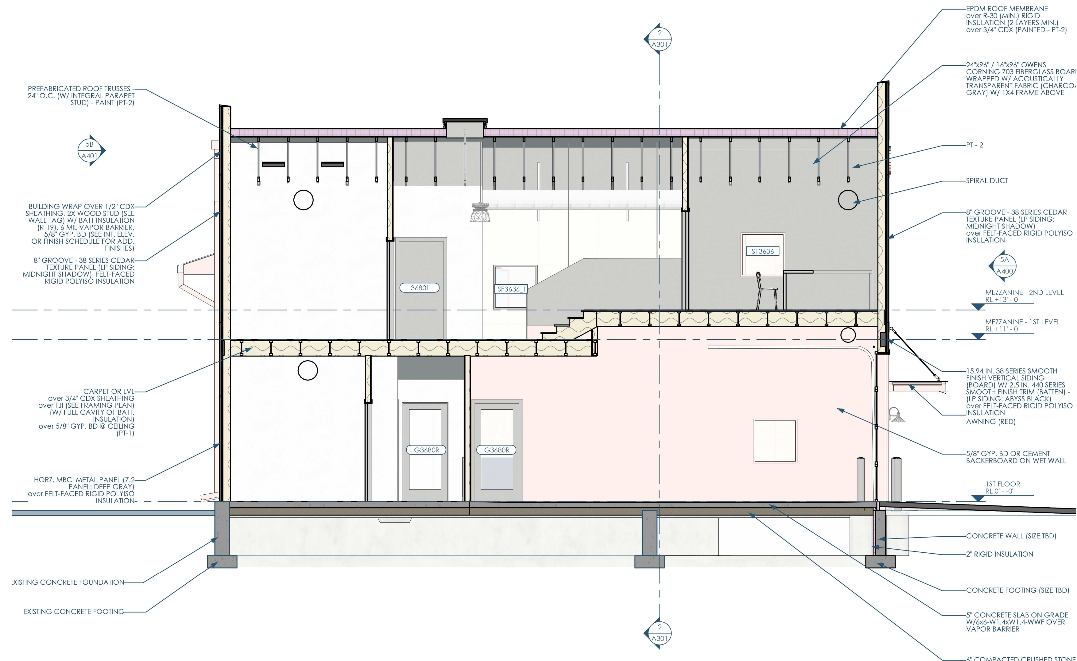
3/A303 SECTION - NS - WEST - AT DROPOFF BAY 1/4"=1'-0"
