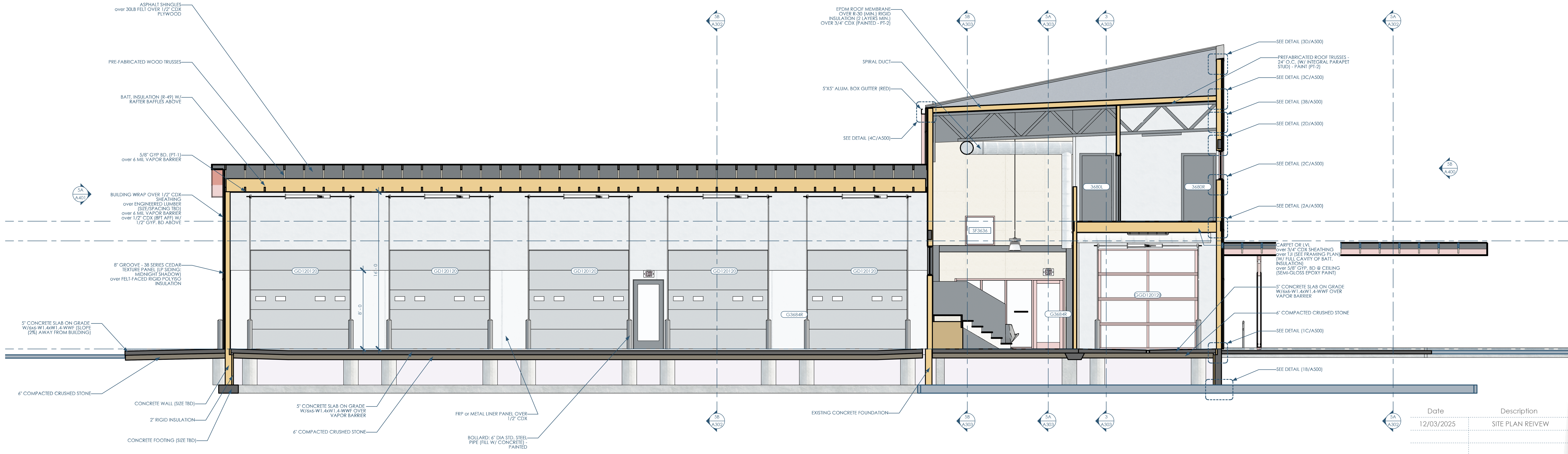
2/A301 SECTION - EW - NORTH 1/4"=1'-0"
