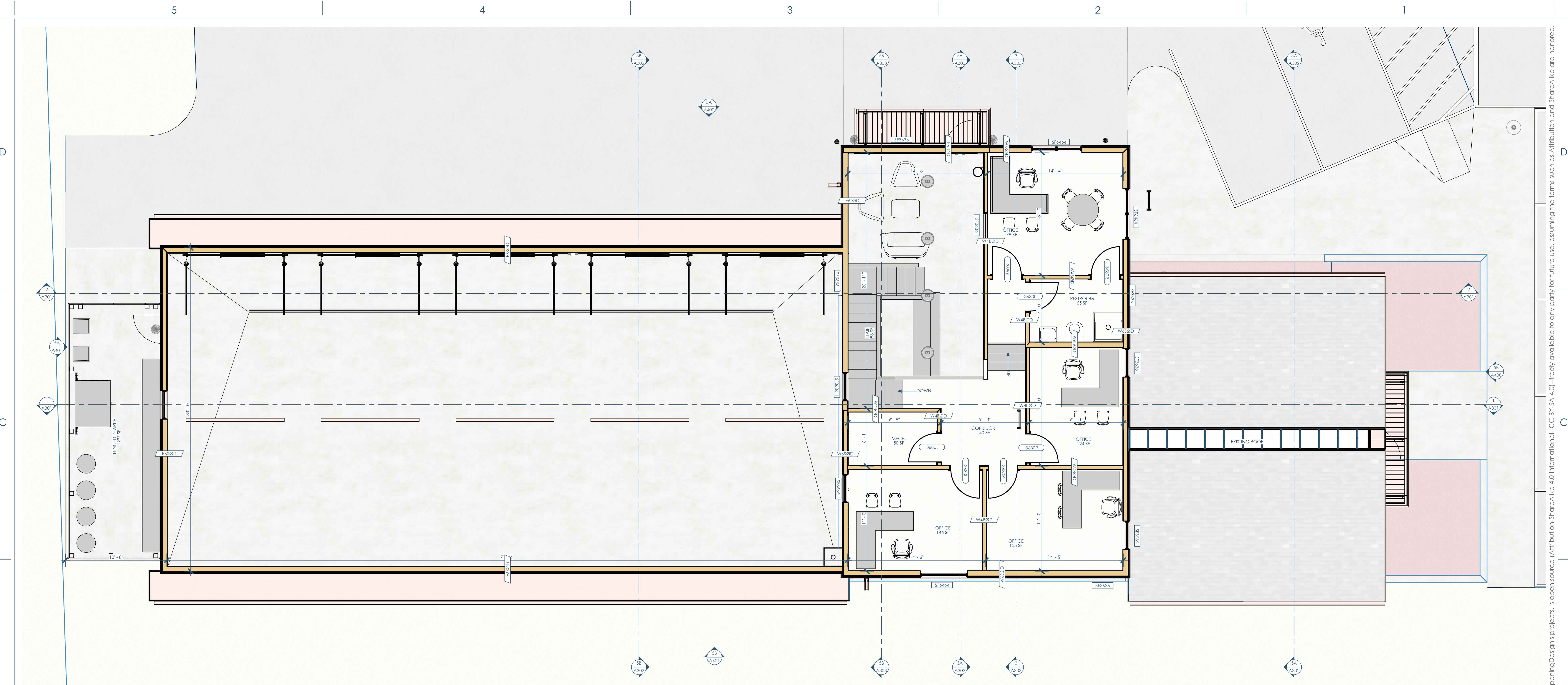
5B/A102 PHASE 2 - MEZZ 1/4"=1'-0"
