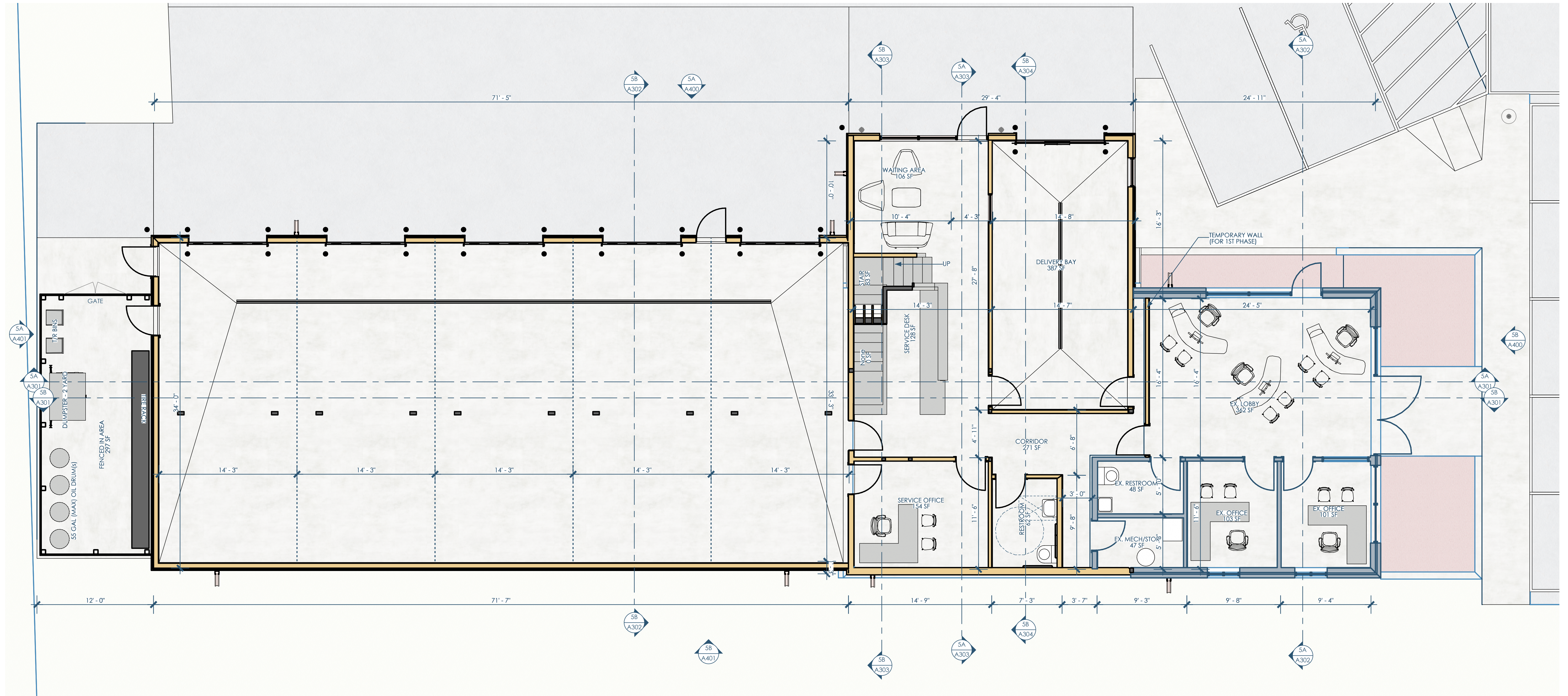
5B/A101 PHASE 1 - 1ST FLOOR 3/16"=1'-0"
