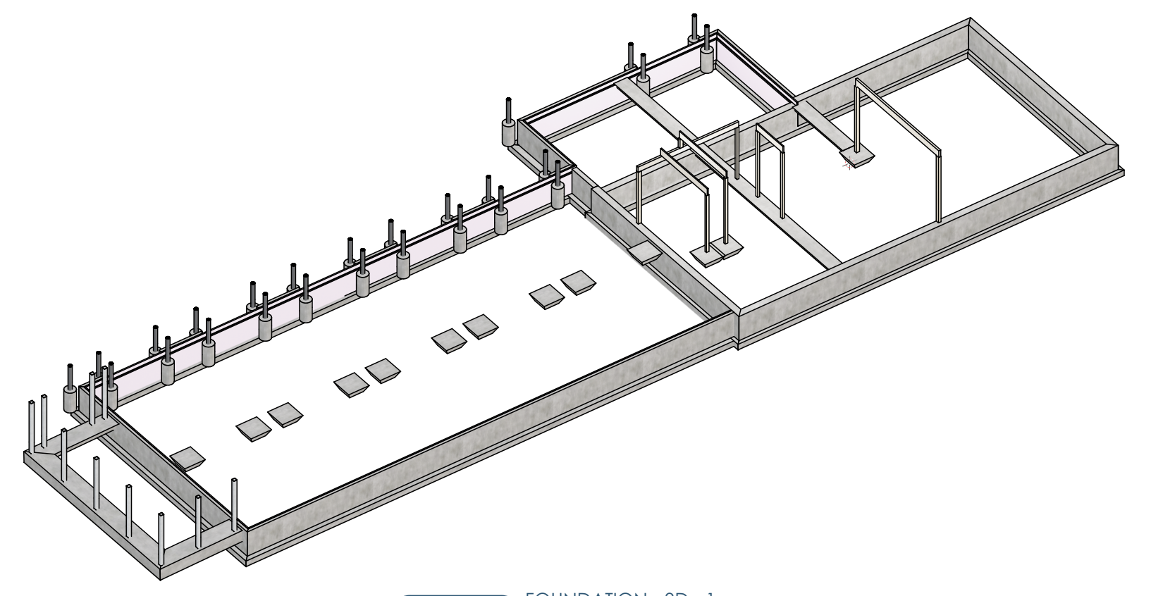
1A/S101 FOUNDATION - 3D - 1 1/16"=1'-0"
