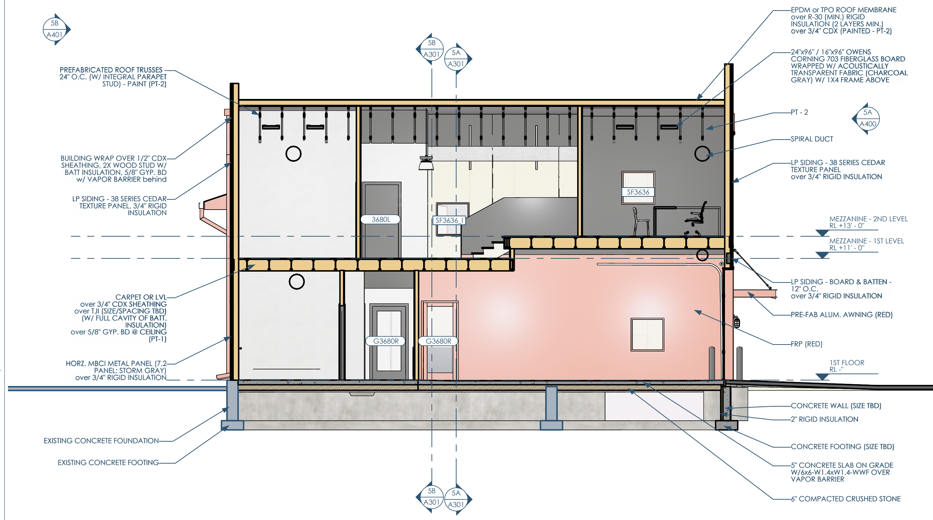
5B/A304 SECTION - NS - WEST - AT DROPOFF BAY 3/16"=1'-0"
