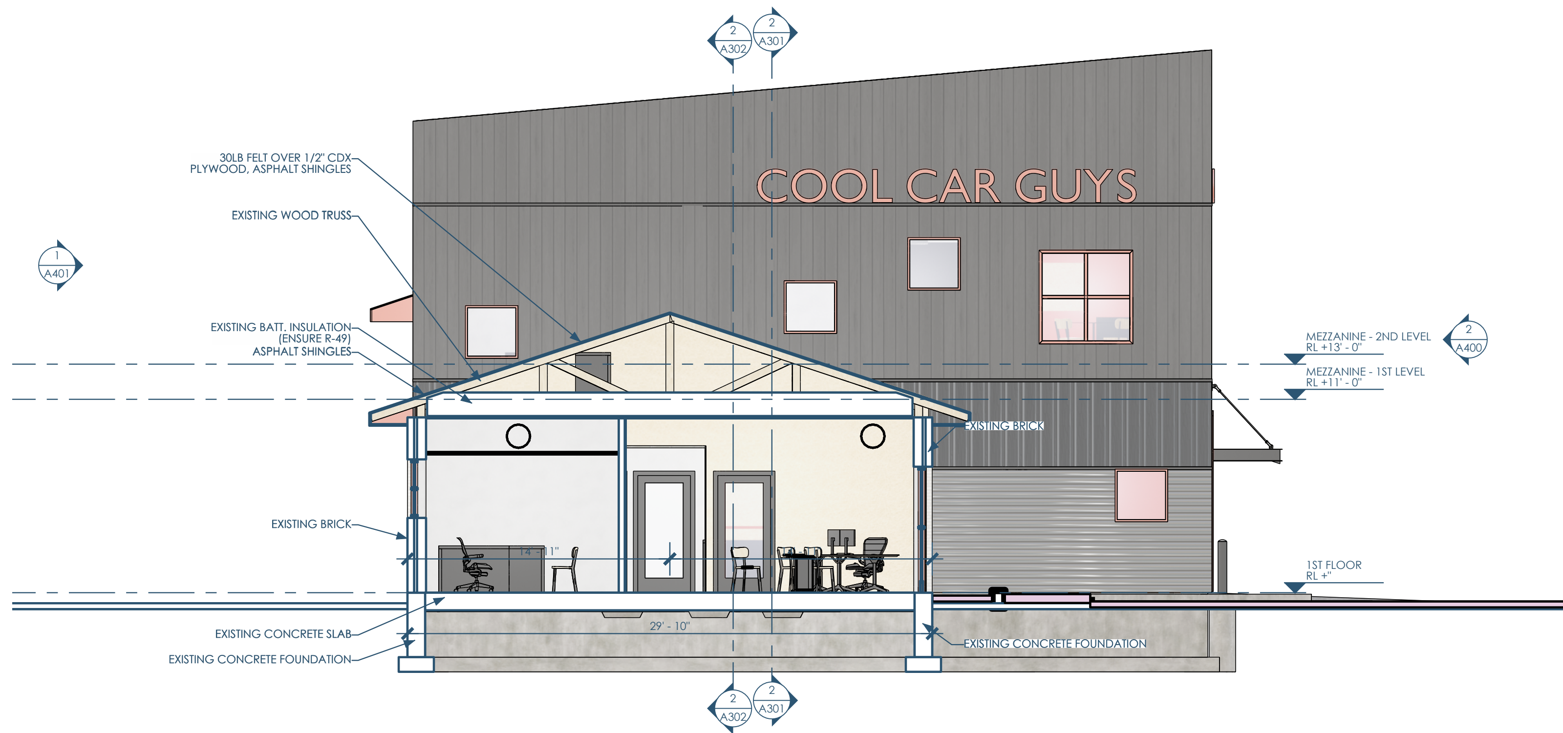
5B/A302 SECTION - NS - EAST - AT SERVICE BAY 3/16"=1'-0"
