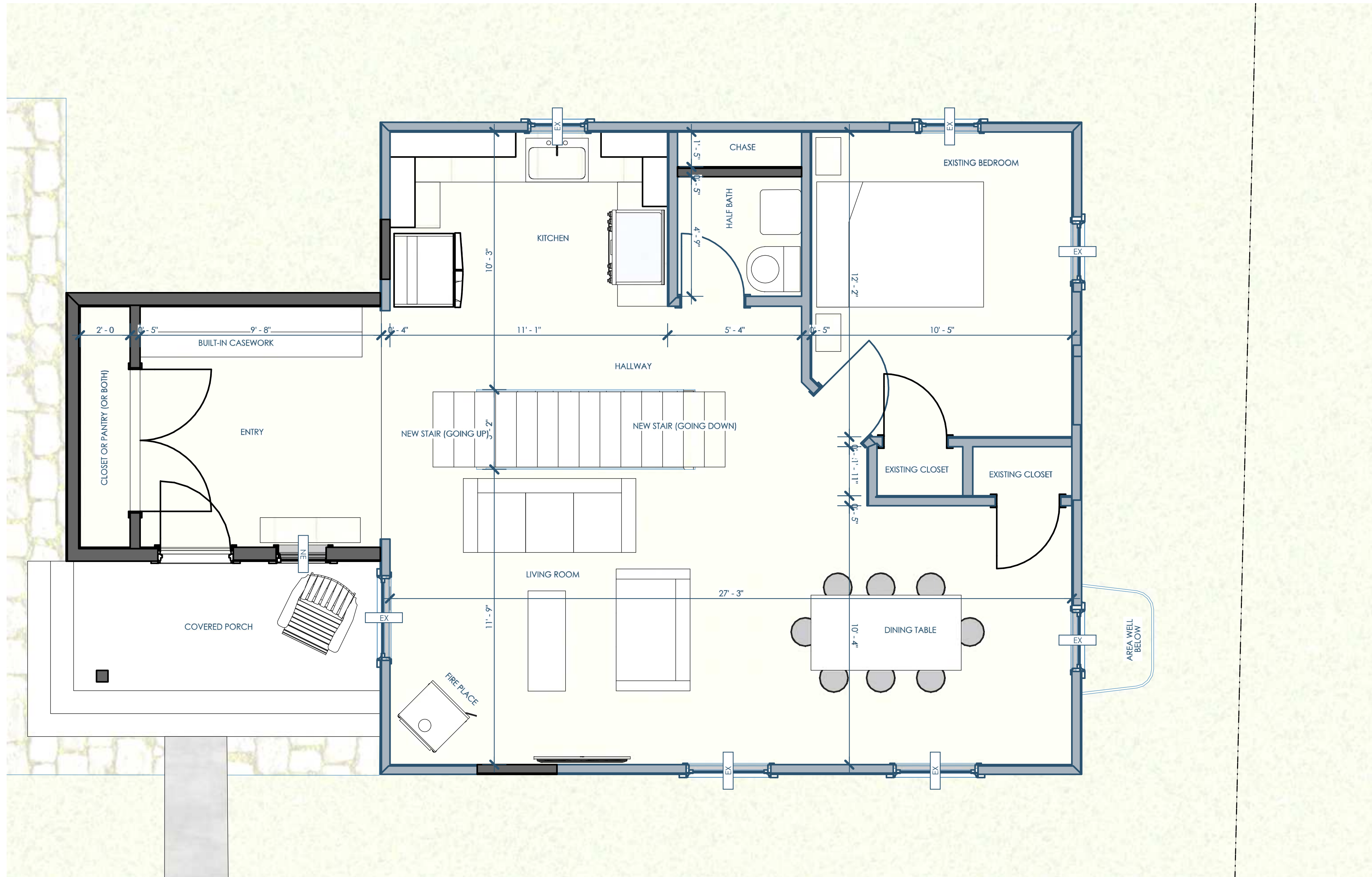
1/A101 O2 - FLOOR PLAN - 1ST FLOOR 3/8"=1'-0"
