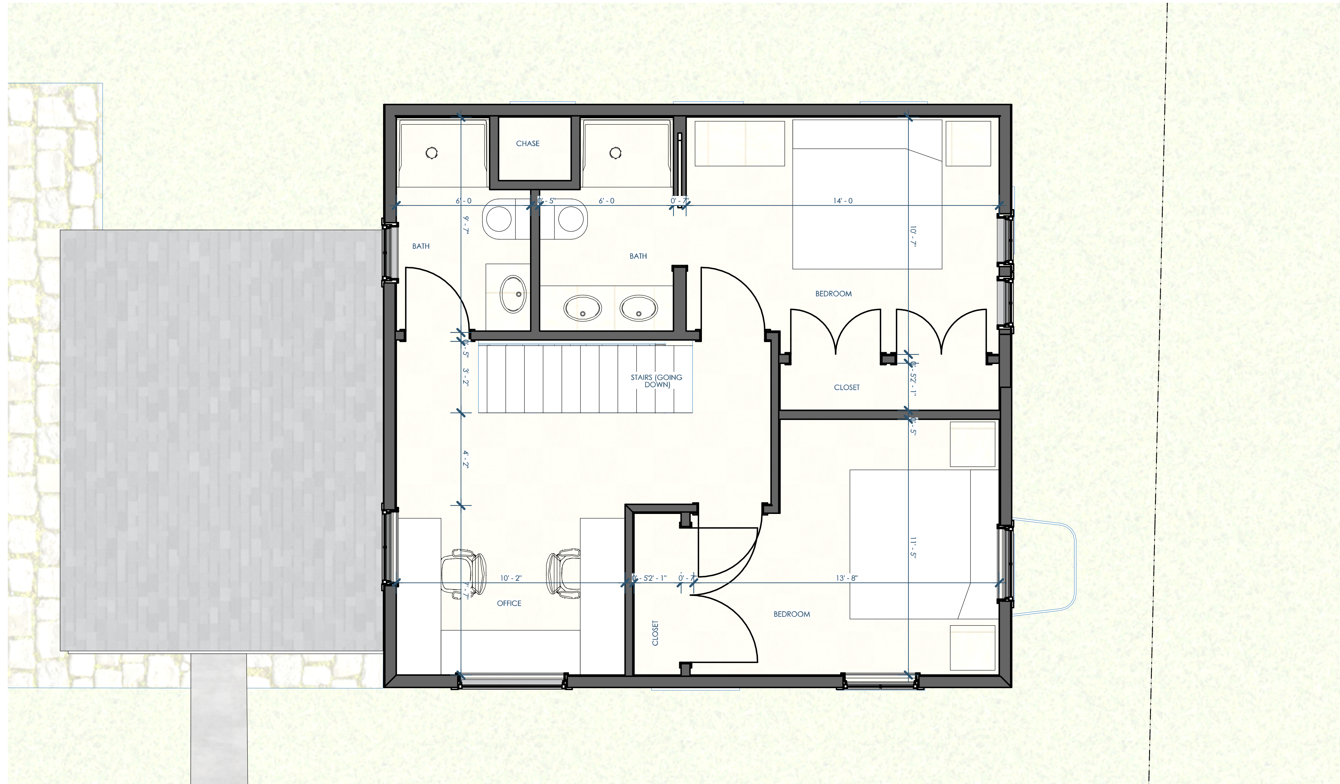
5B/A102 O2 - FLOOR PLAN - 2ND FLOOR 3/8"=1'-0"
