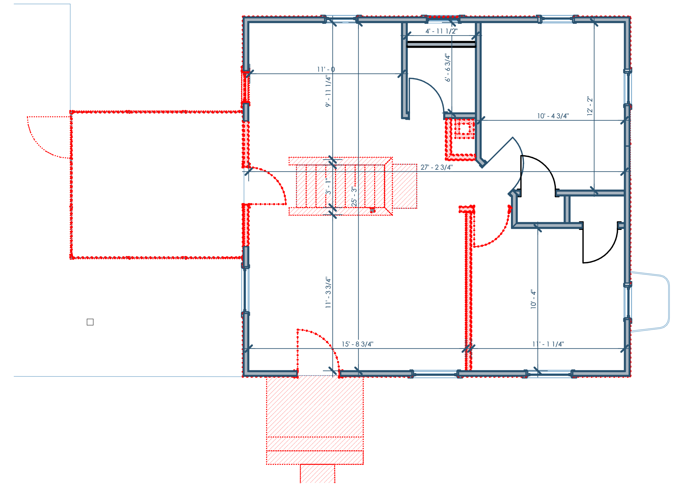
2B/A000 DEMOLITION PLAN 1/4"=1'-0"
