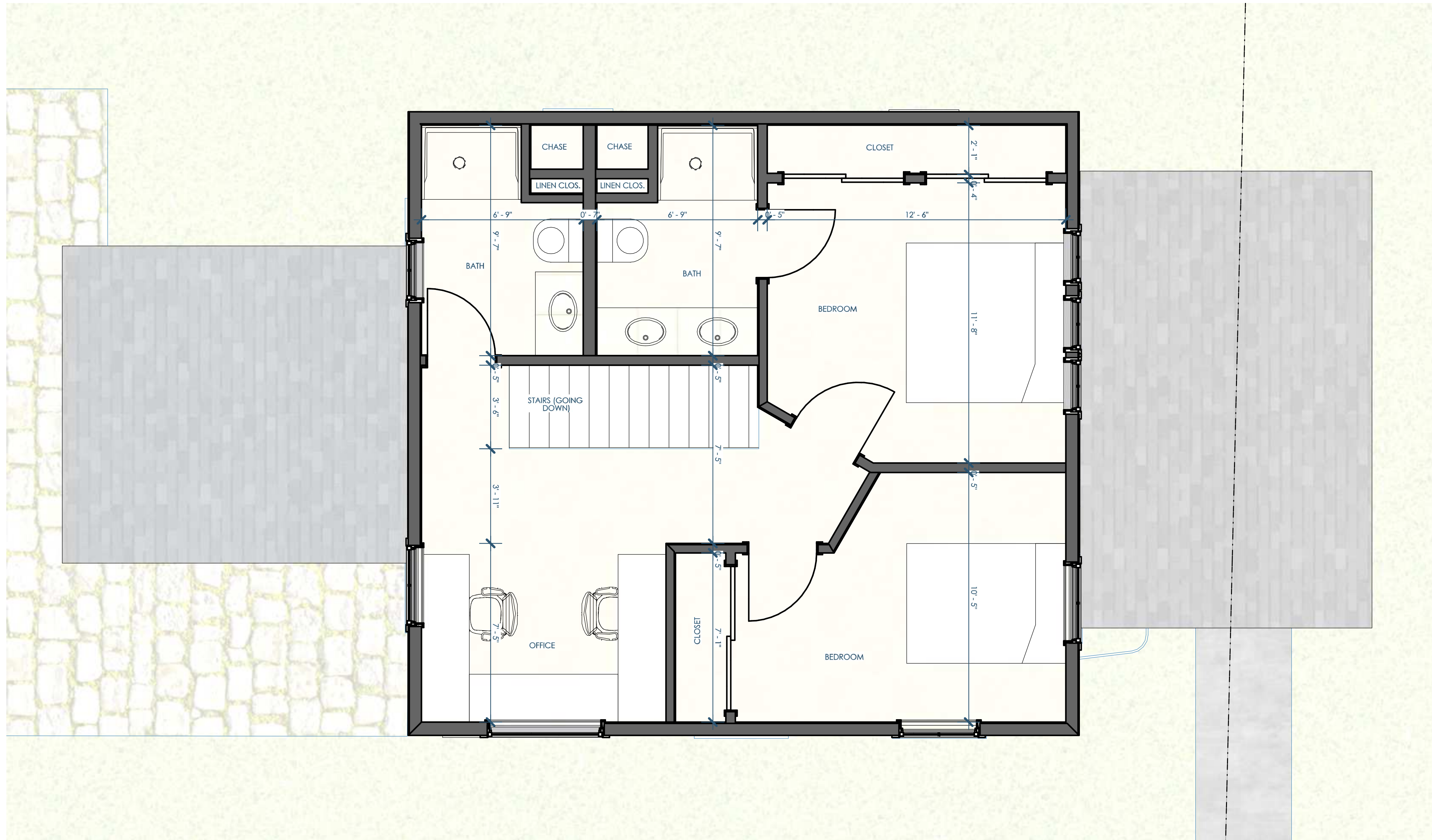
5B/A102 FLOOR PLAN - 2ND FLOOR 3/8"=1'-0"
