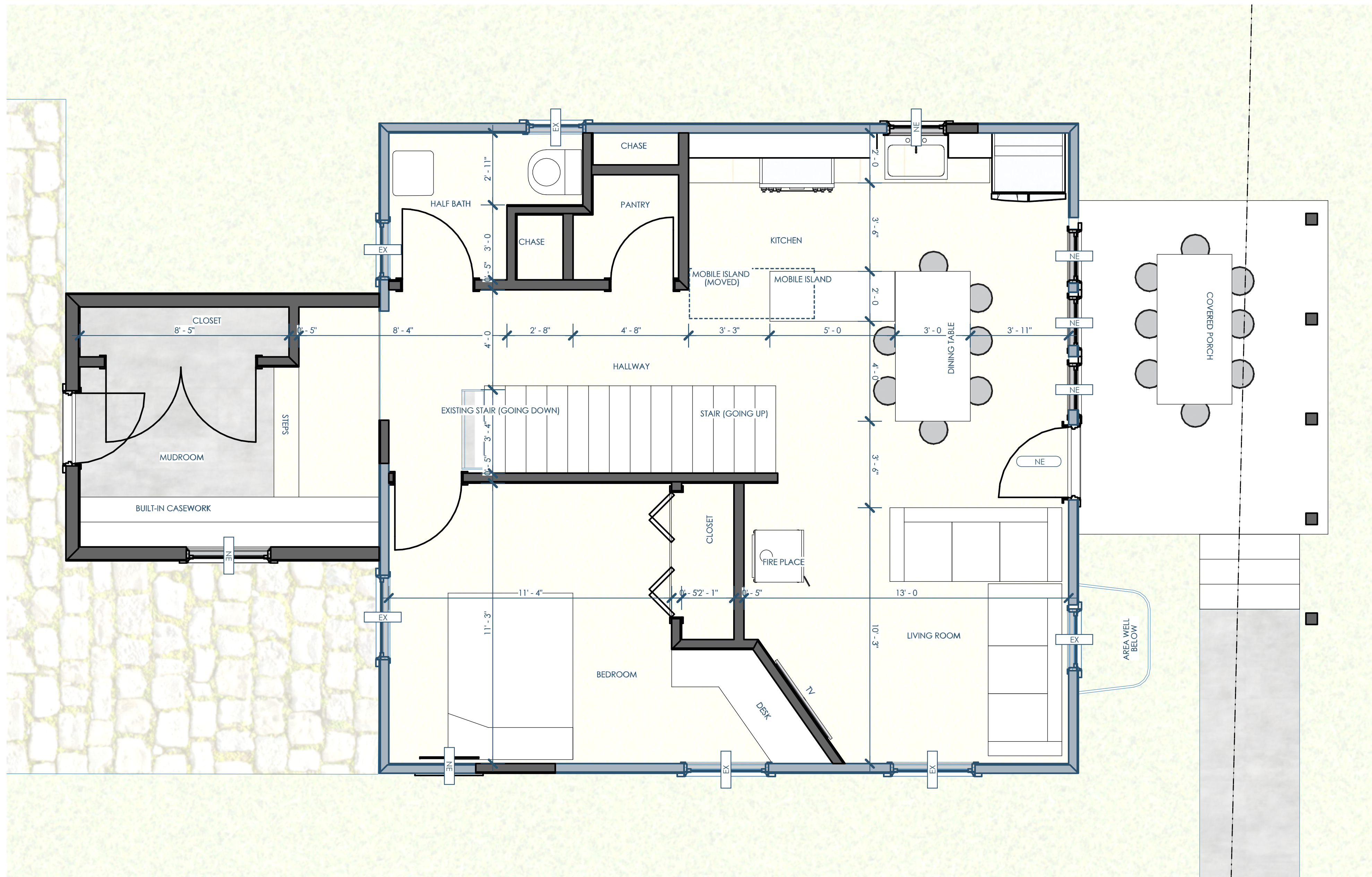
5B/A101 FLOOR PLAN - 1ST FLOOR 3/8"=1'-0"
