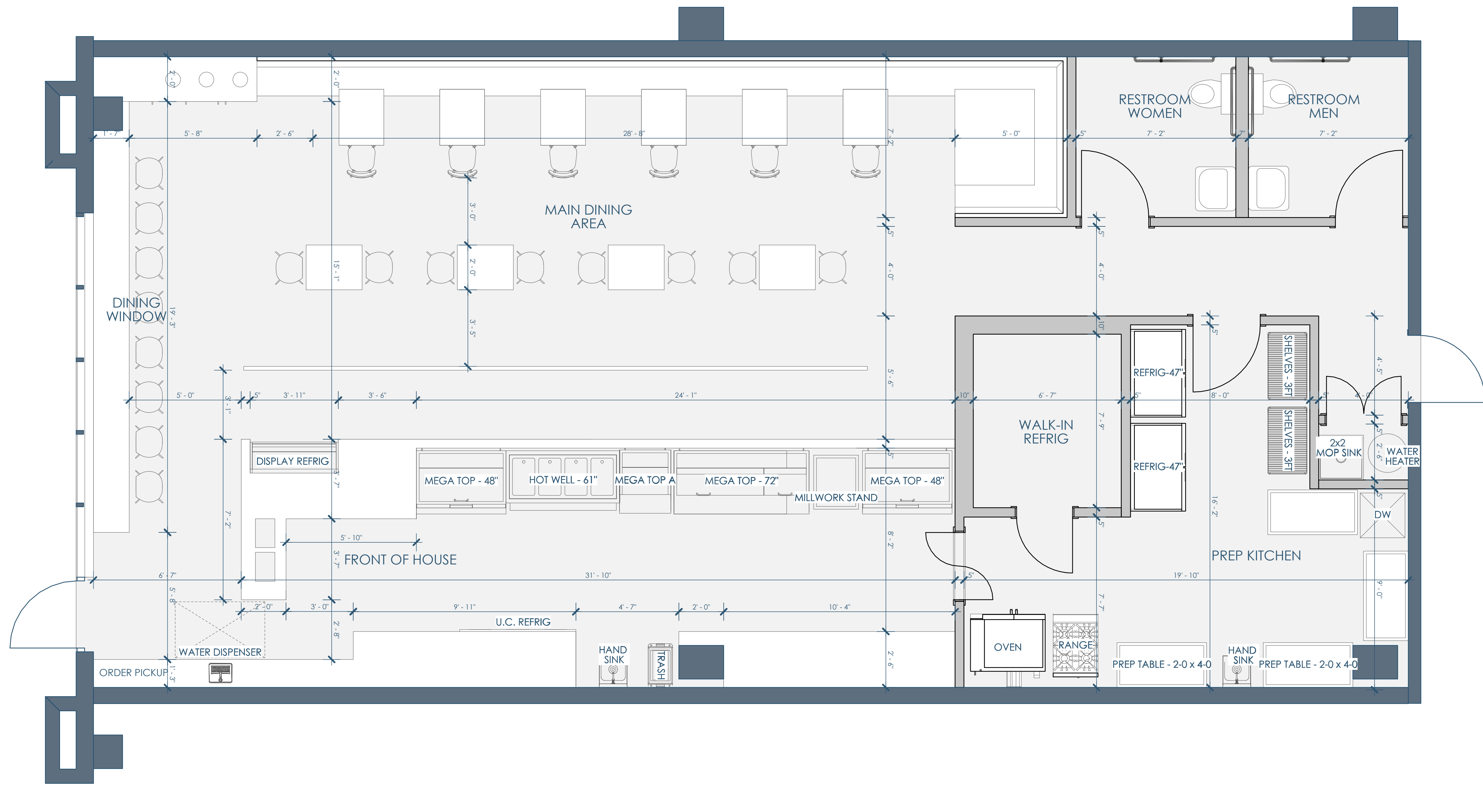
5A/A101 FLOOR PLAN - 1ST FLOOR 3/8"=1'-0"
