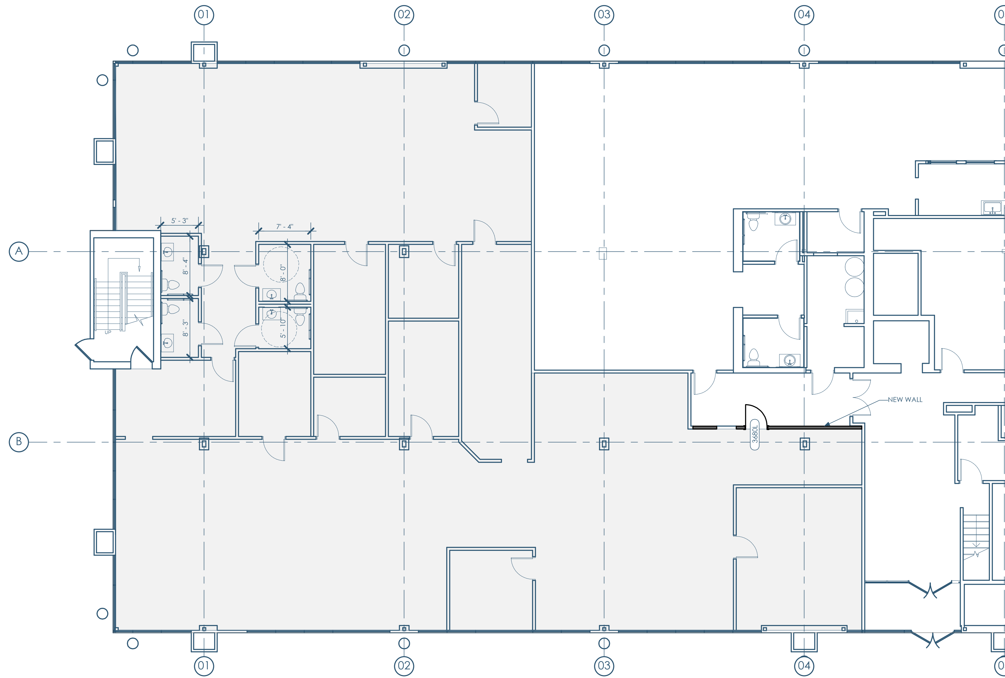
1/A100 FLOOR PLAN - 1ST FLOOR 1/8"=1'-0"
