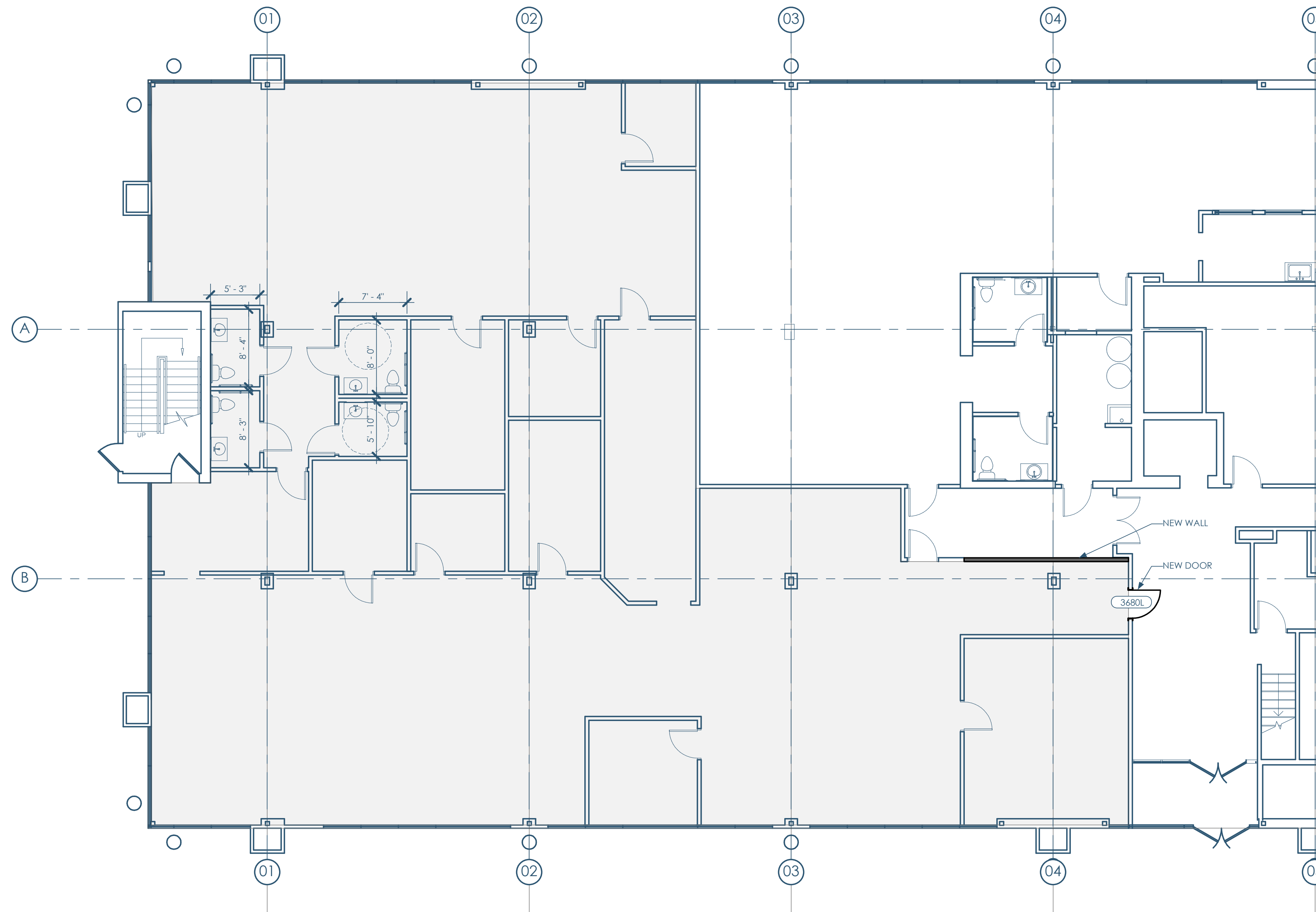
1/A100 FLOOR PLAN - 1ST FLOOR 1/8"=1'-0"
