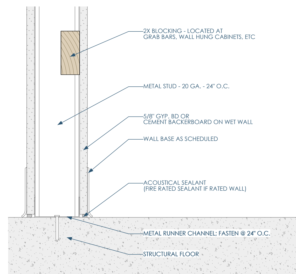
3A/A000 W1 - FULL HEIGHT PARTITION - NOT RATED - BASE 3\"/>
